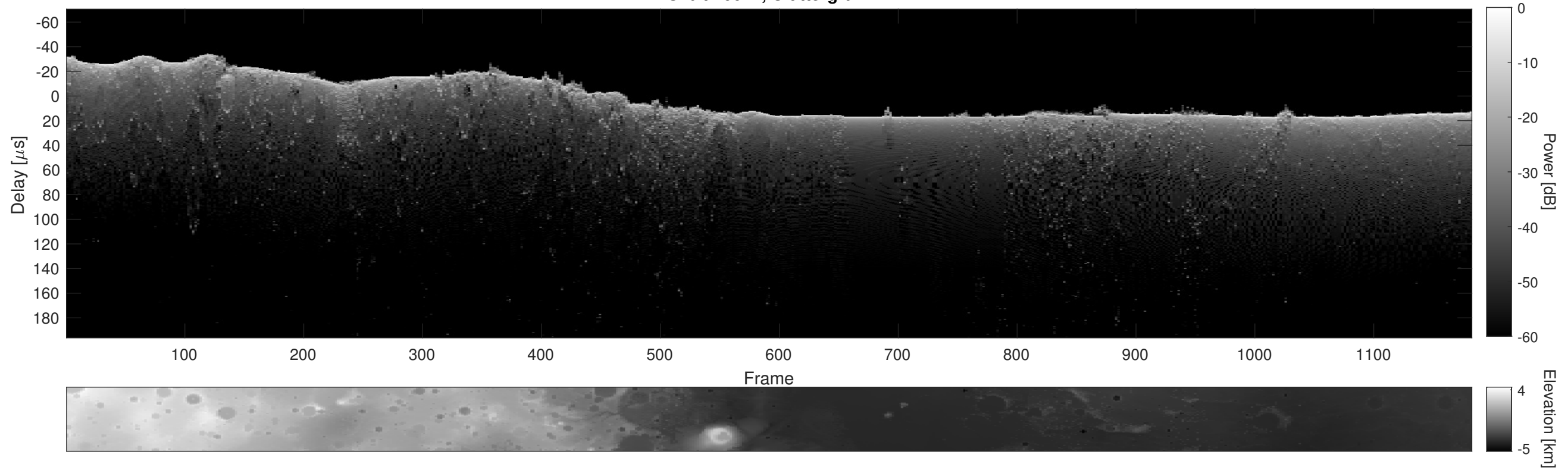
Orbit 16611, Cluttergram
