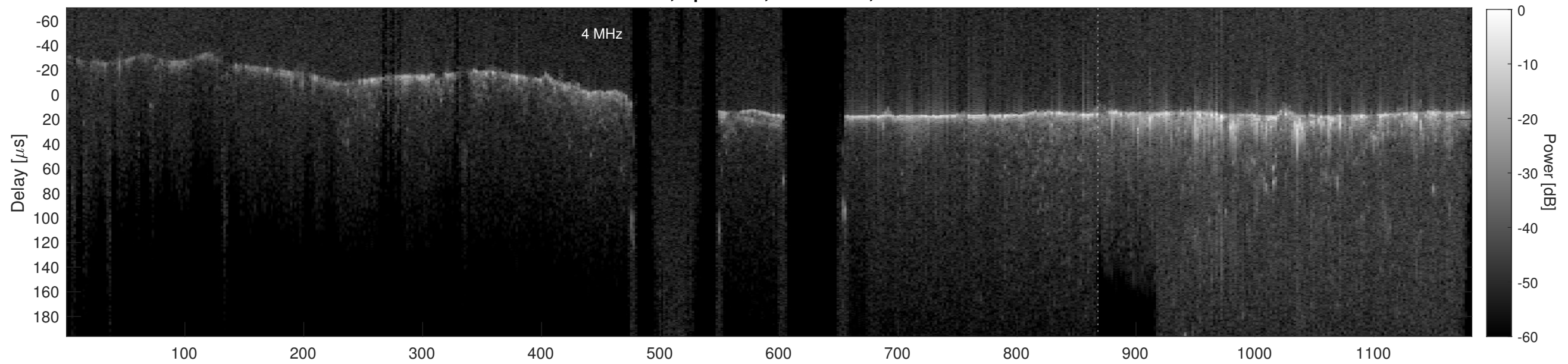
Orbit 16611, Cluttergram
