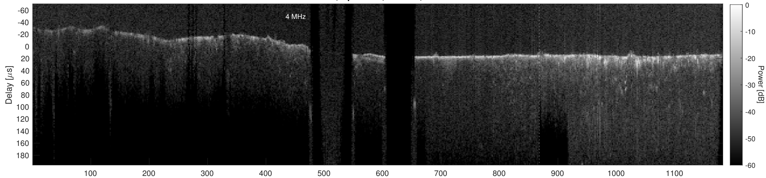
Orbit 16611, Cluttergram
