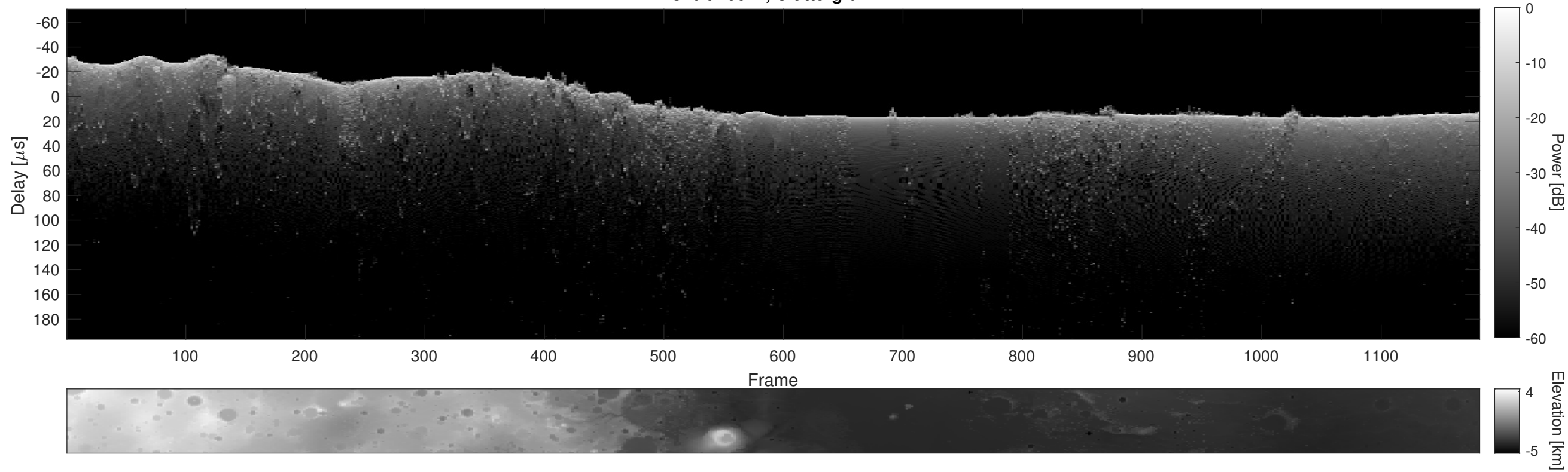
Orbit 16611, Cluttergram
