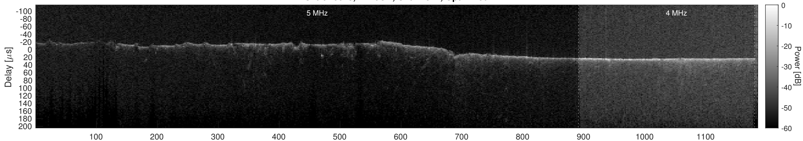
Orbit 16615, Cluttergram
