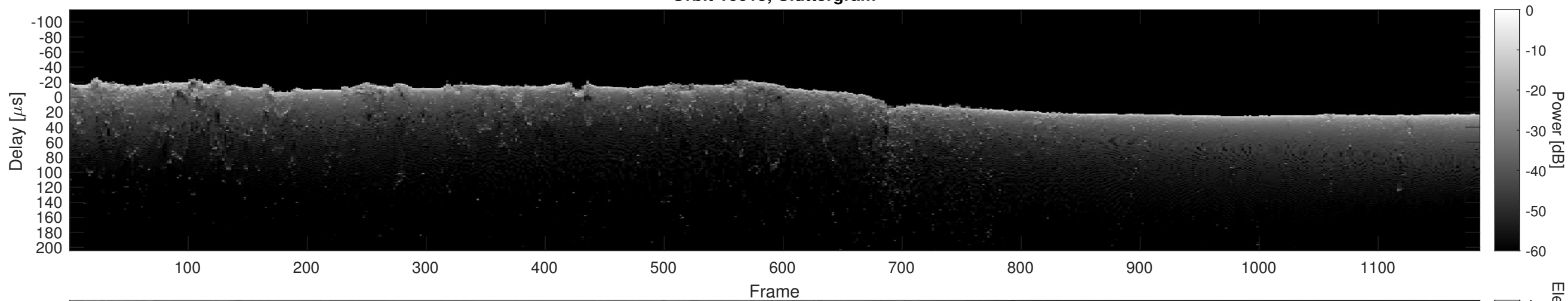
Orbit 16615, Cluttergram
