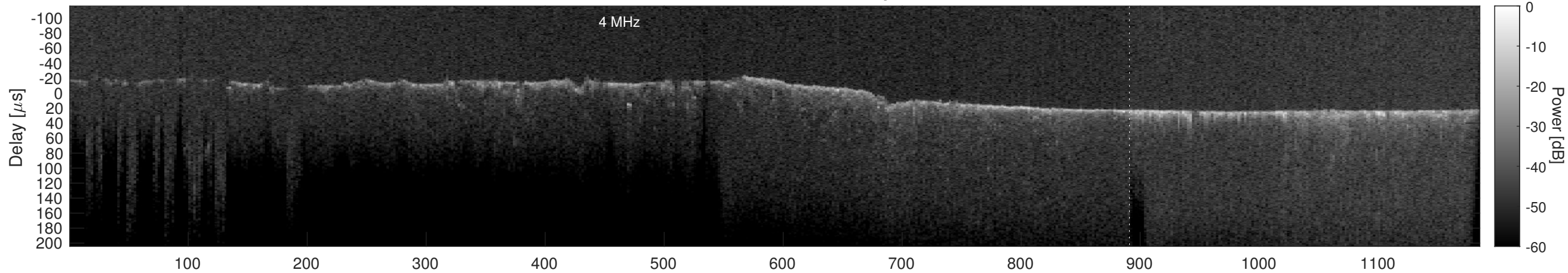
Orbit 16615, Cluttergram
