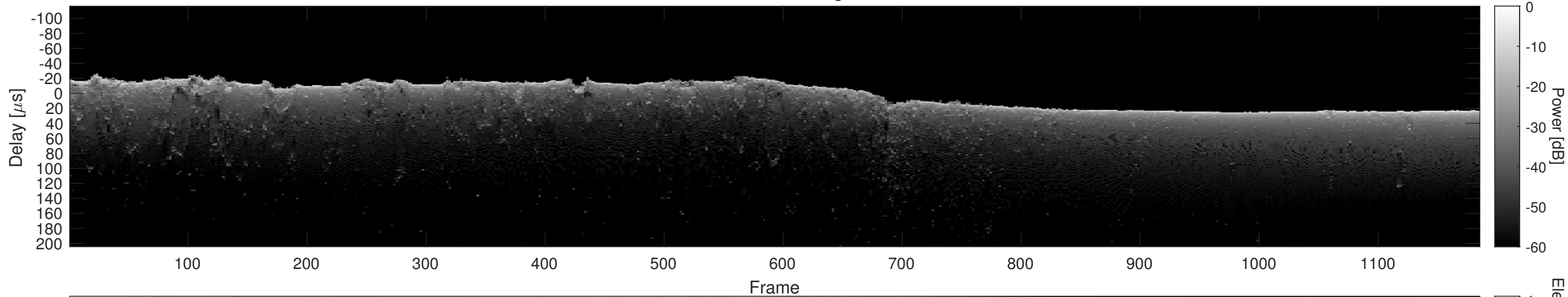
Orbit 16615, Cluttergram
