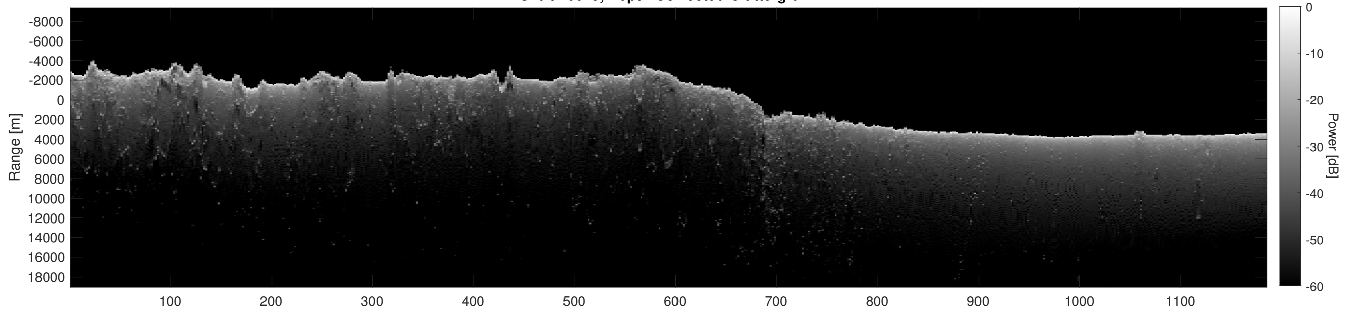
Orbit 16615, Depth-Corrected Cluttergram
