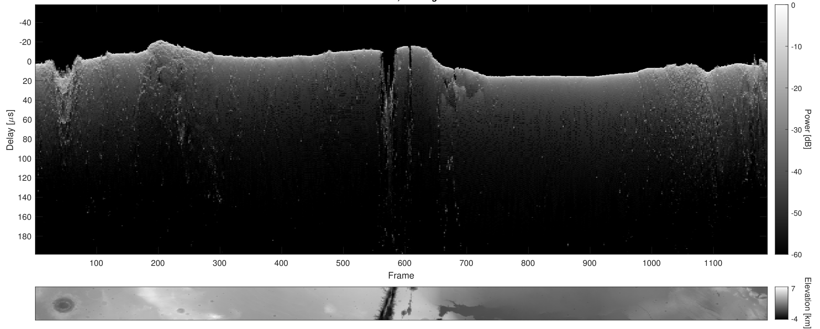
Orbit 16617, Cluttergram
