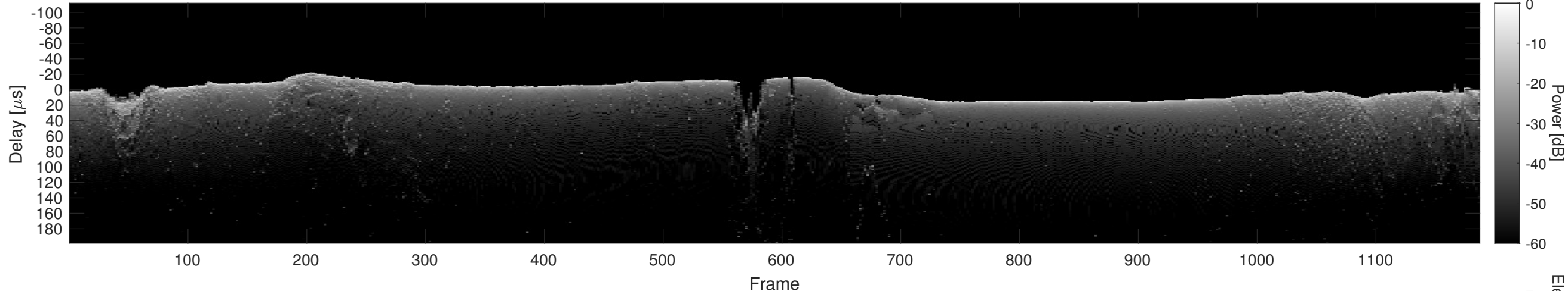
Orbit 16617, Cluttergram
