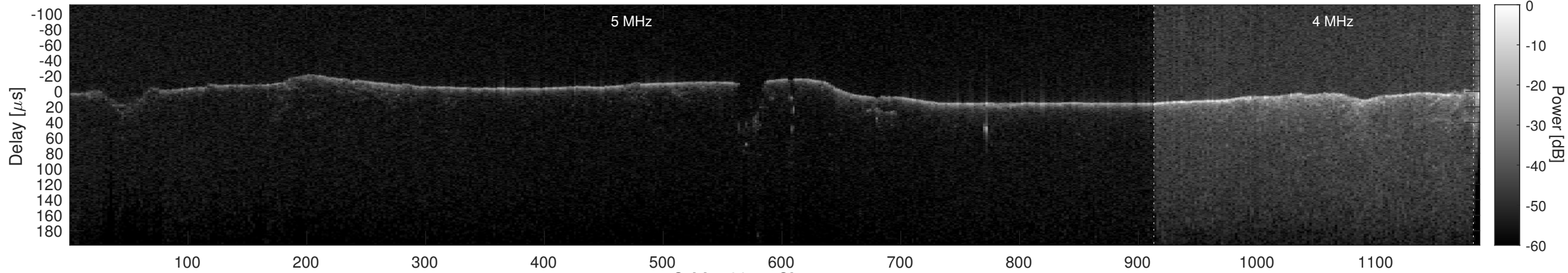
Orbit 16617, Cluttergram
