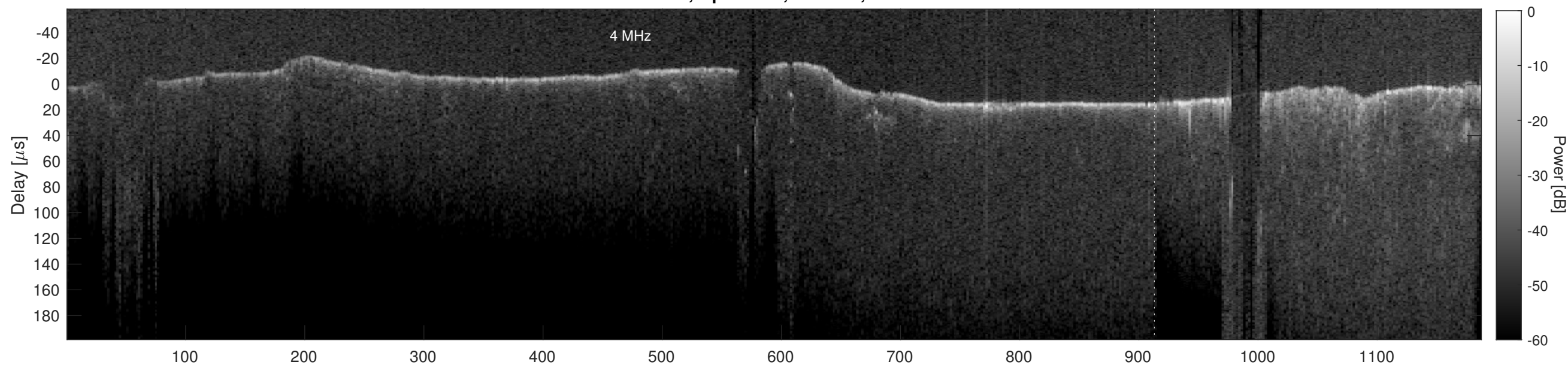
Orbit 16617, Cluttergram
