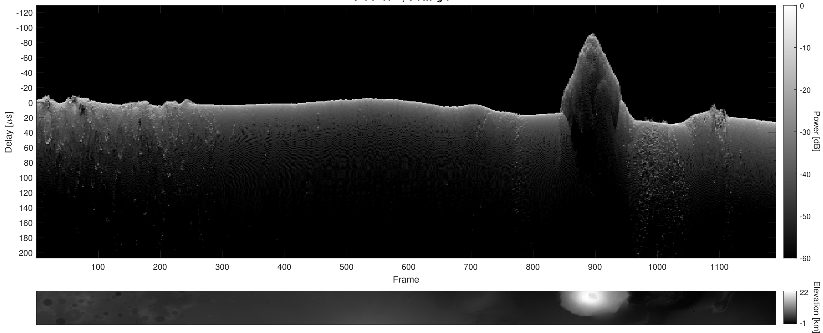
Orbit 16621, Cluttergram
