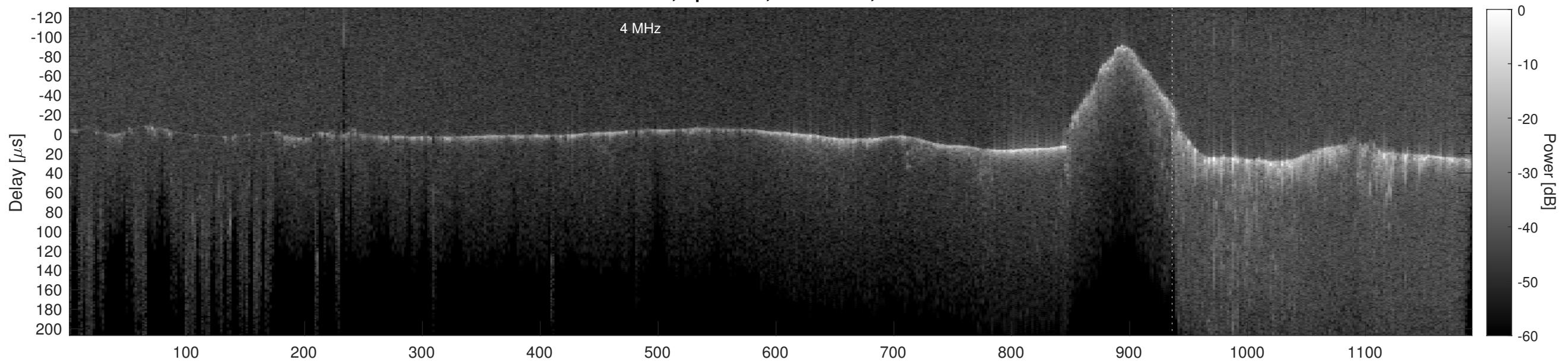
Orbit 16621, Cluttergram
