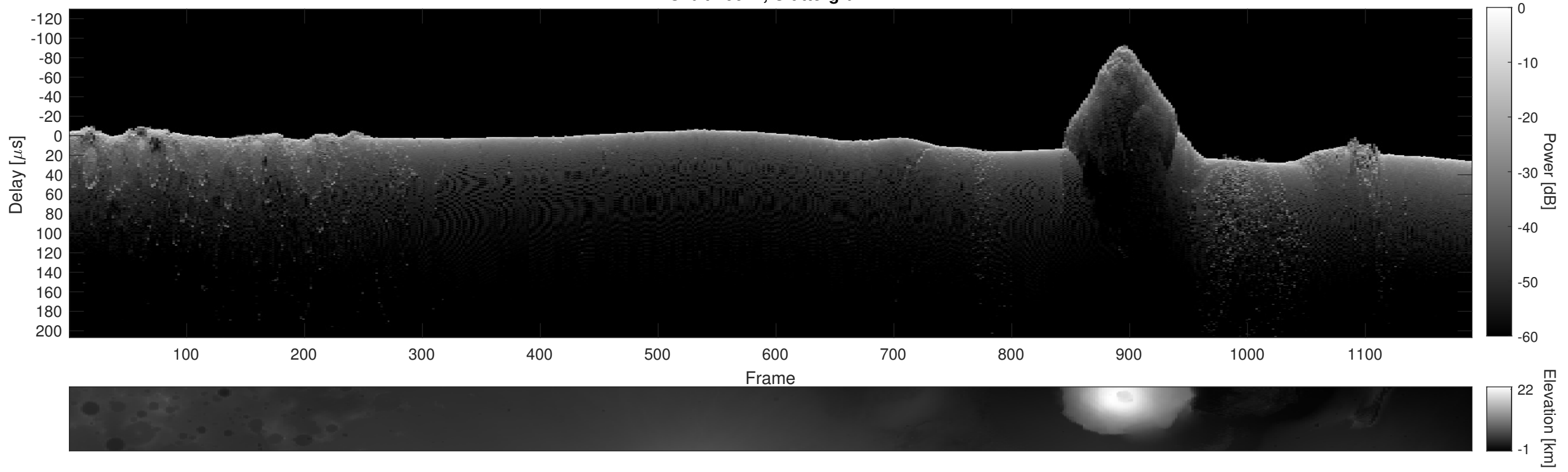
Orbit 16621, Cluttergram
