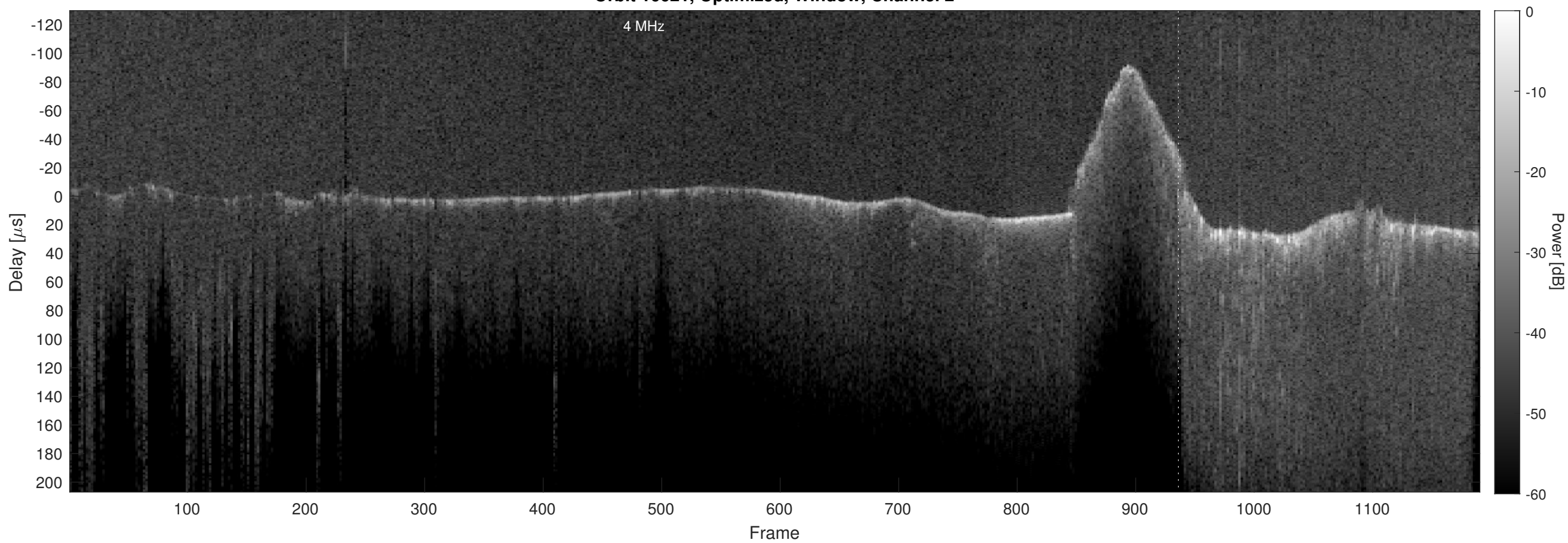
Orbit 16621, Optimized, Window, Channel 2
