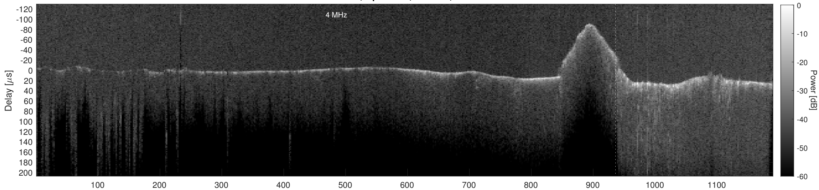
Orbit 16621, Cluttergram
