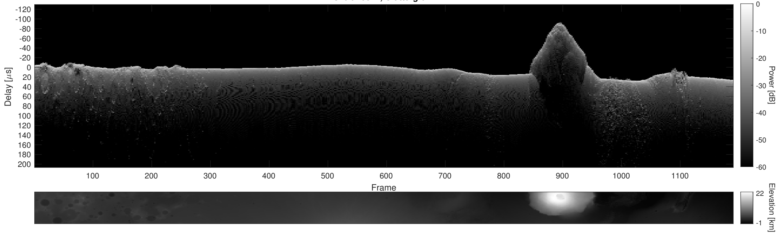
Orbit 16621, Cluttergram
