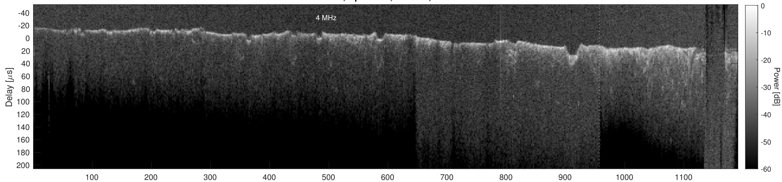
Orbit 16623, Cluttergram
