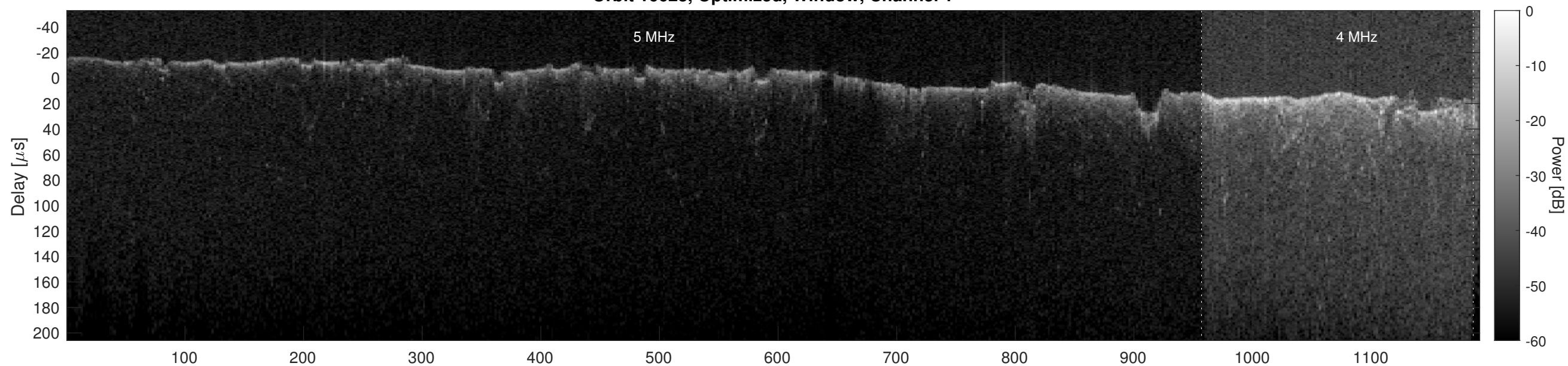
Orbit 16623, Optimized, Window, Channel 2
