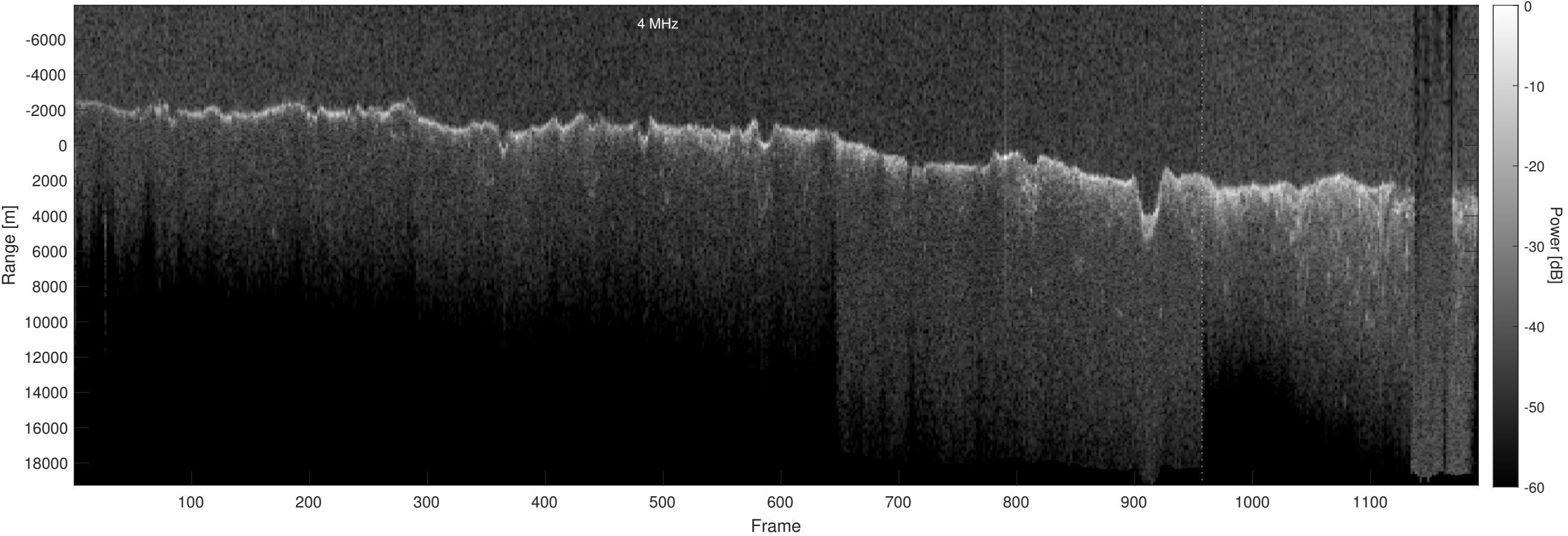
Orbit 16623, Optimized, Window, Depth-Corrected, Channel 2
