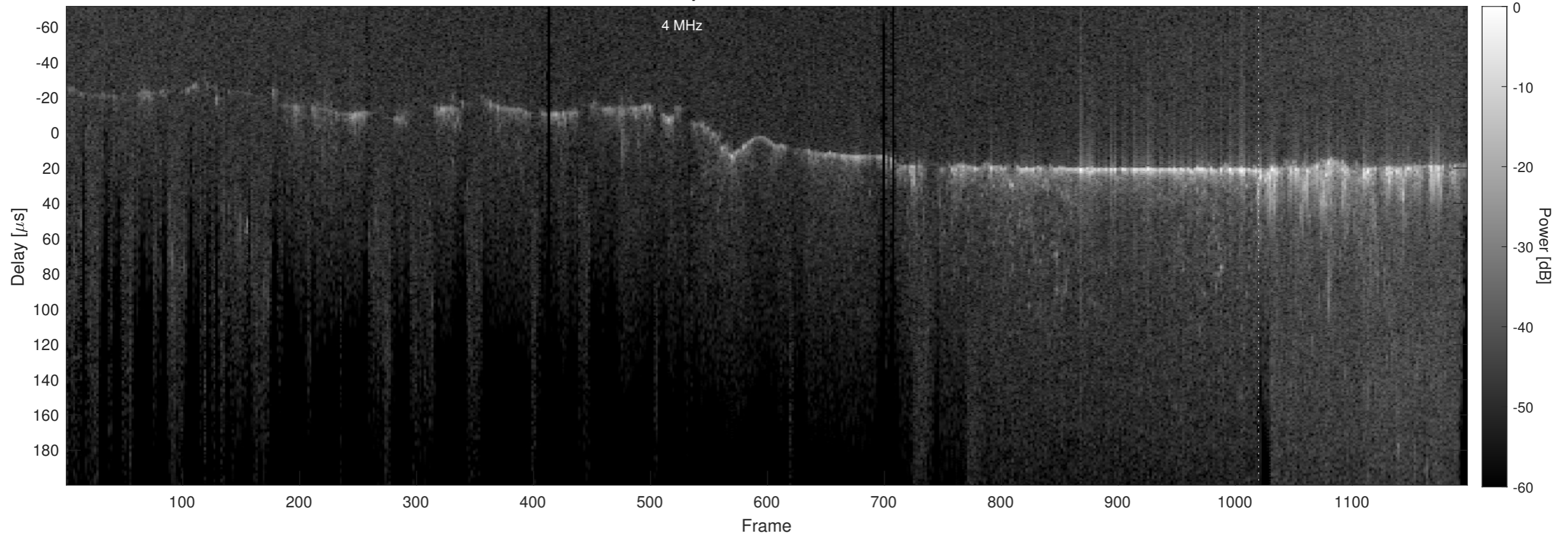
Orbit 16632, Optimized, No Window, Channel 2
