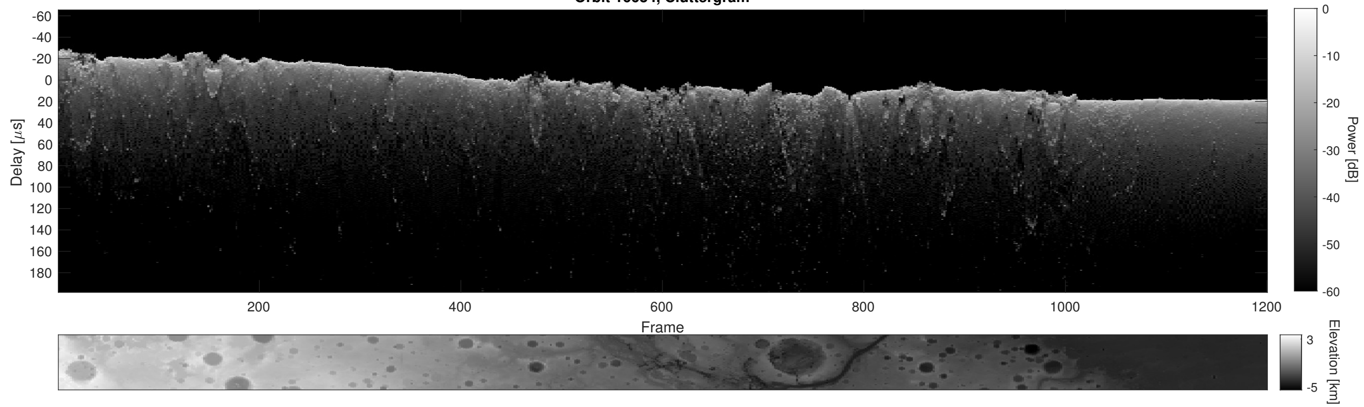
Orbit 16634, Cluttergram
