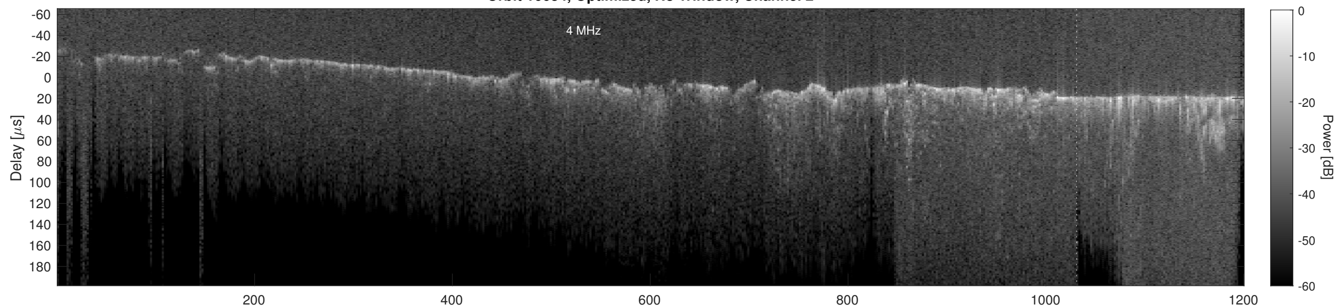
Orbit 16634, Cluttergram
