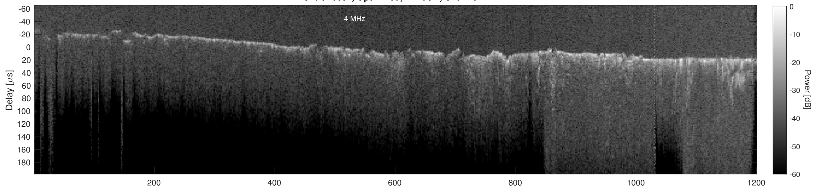
Orbit 16634, Cluttergram
