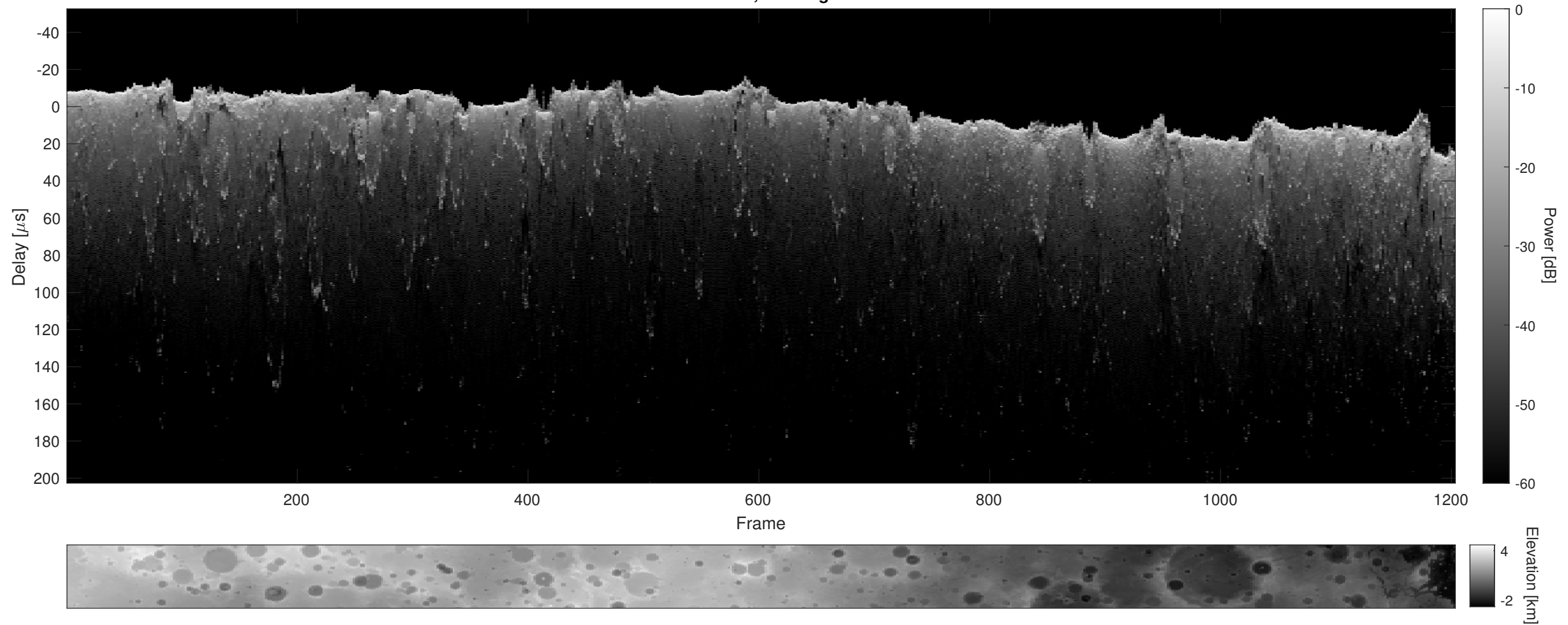
Orbit 16637, Cluttergram
