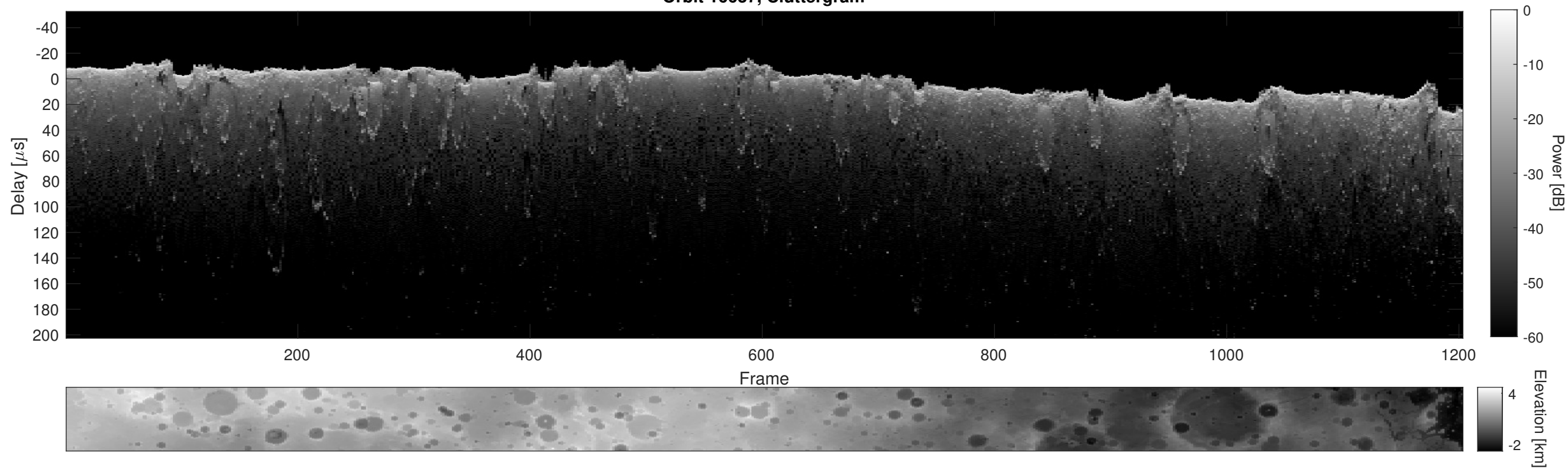
Orbit 16637, Cluttergram
