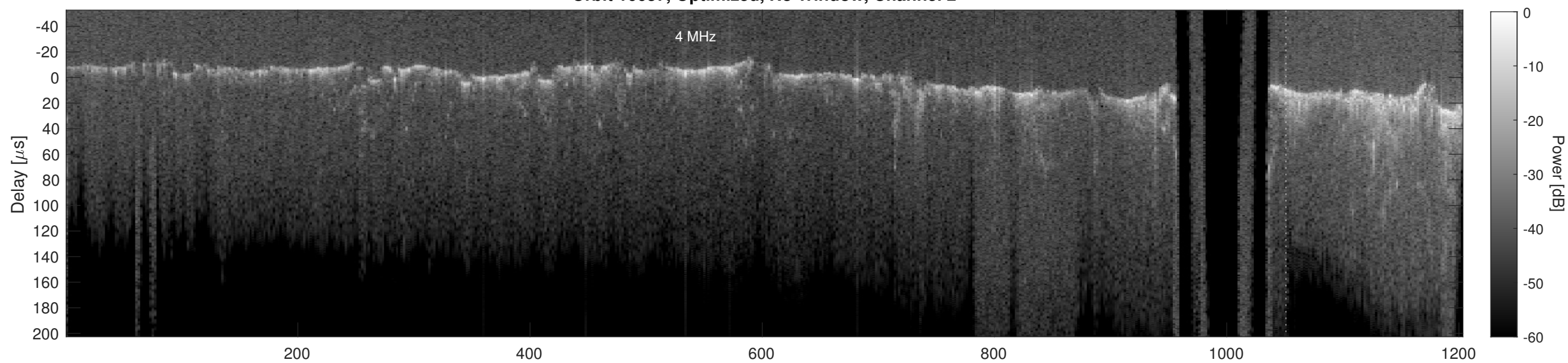
Orbit 16637, Cluttergram
