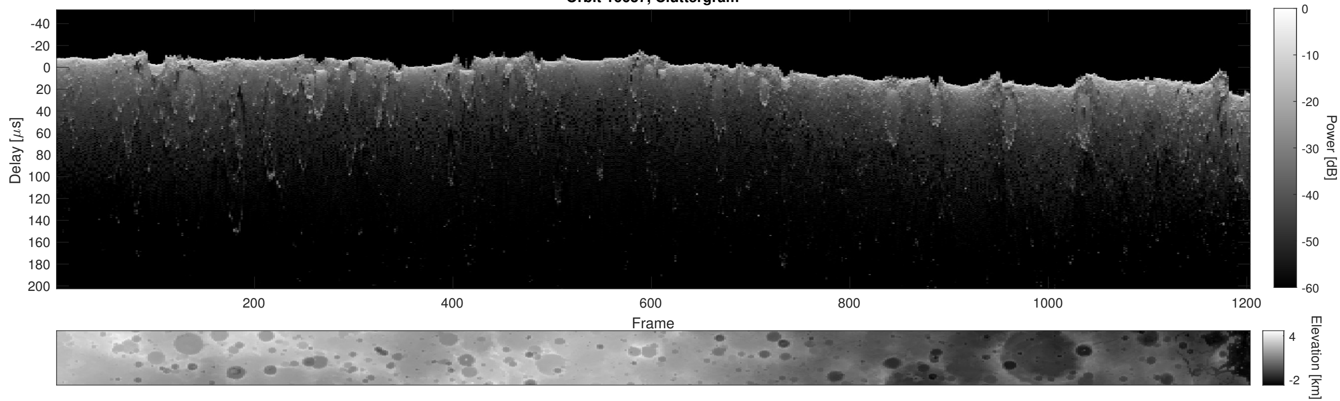
Orbit 16637, Cluttergram
