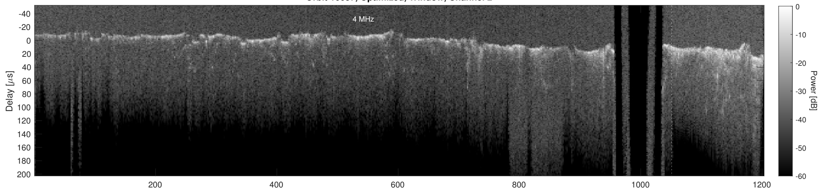
Orbit 16637, Cluttergram
