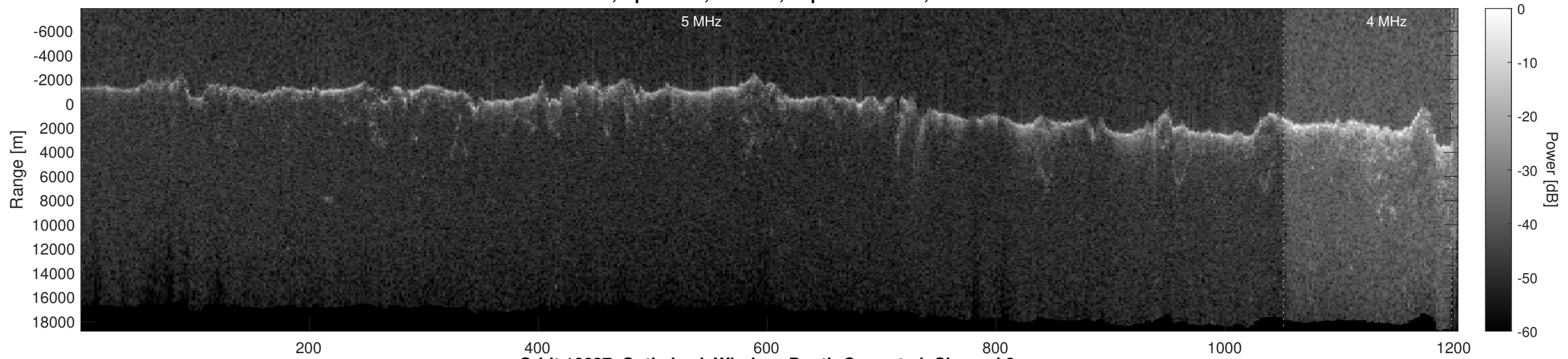
Orbit 16637, Optimized, Window, Depth-Corrected, Channel 2
