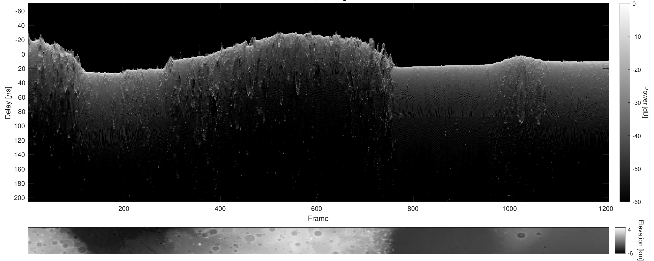
Orbit 16640, Cluttergram
