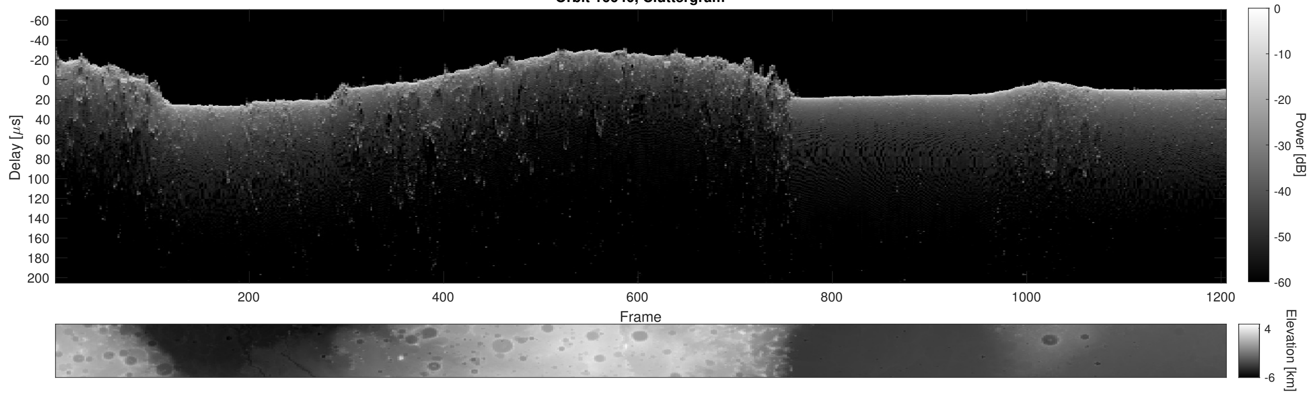
Orbit 16640, Cluttergram
