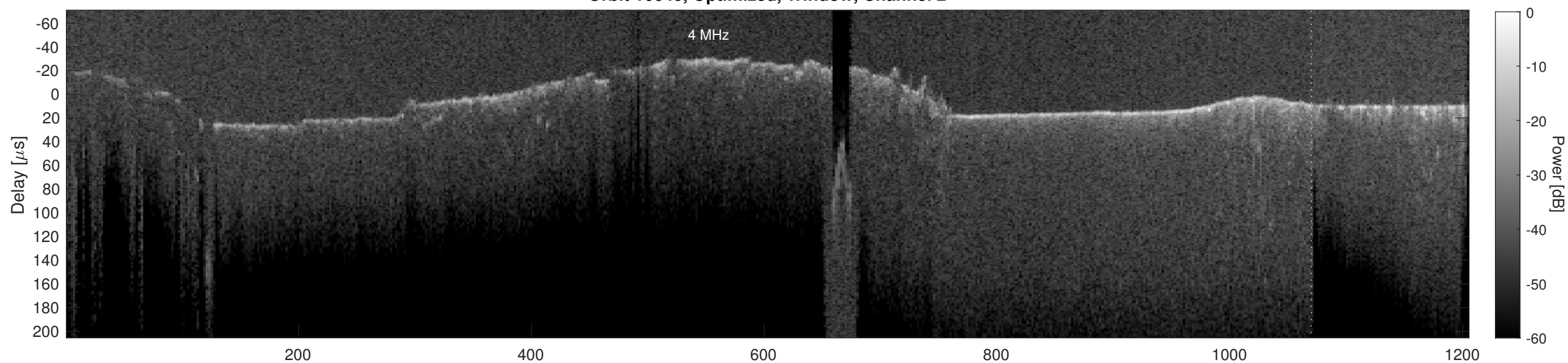
Orbit 16640, Cluttergram
