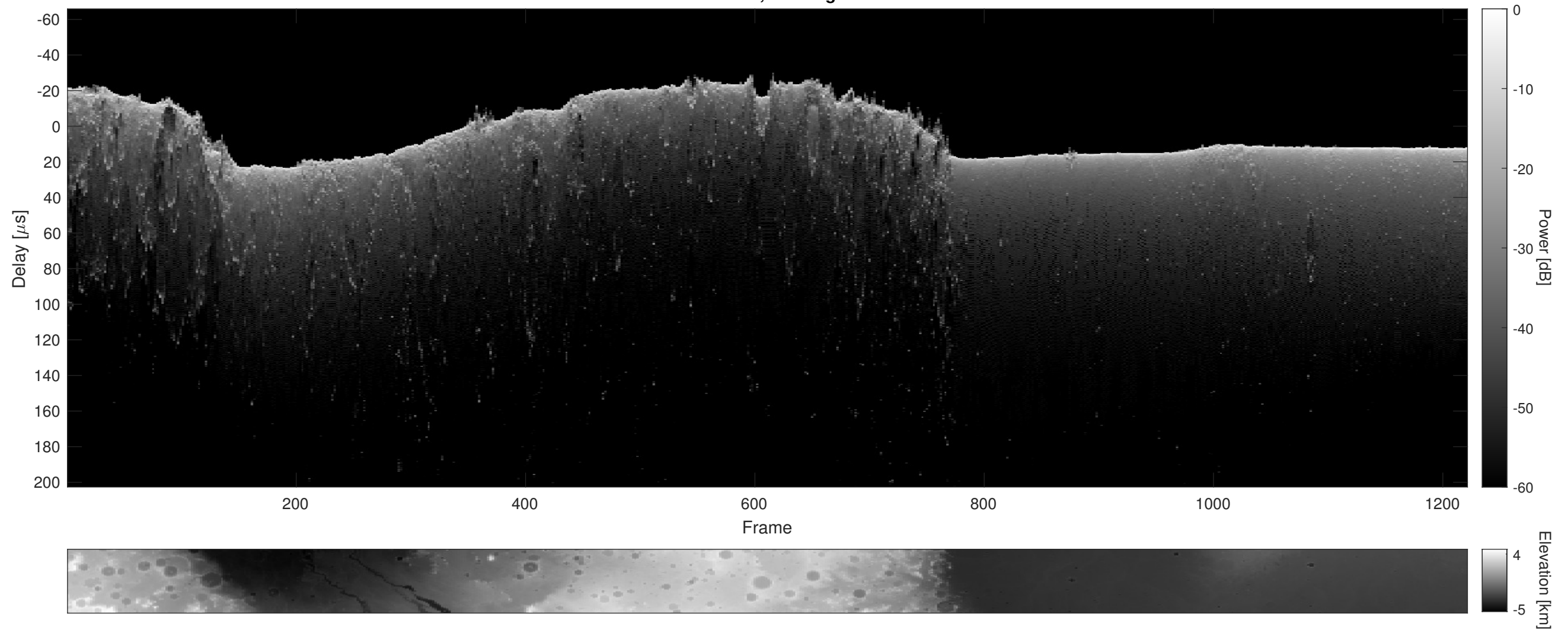
Orbit 16647, Cluttergram
