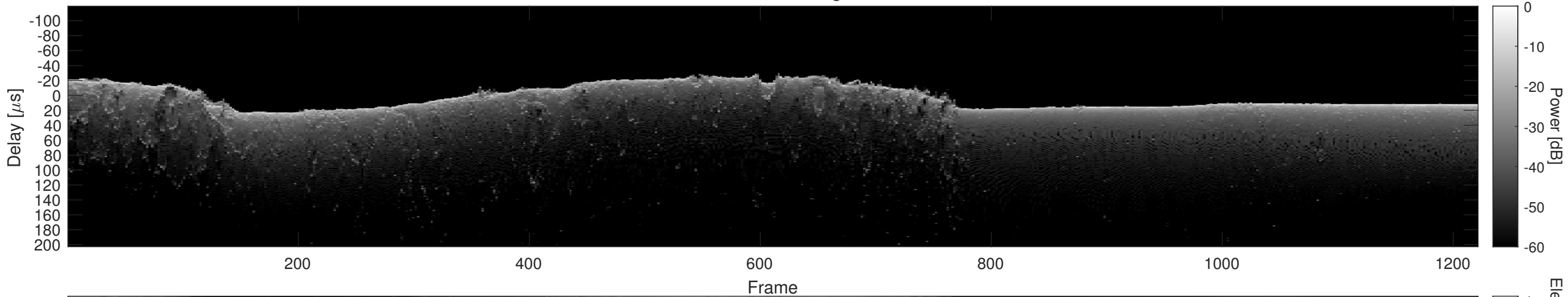
Orbit 16647, Cluttergram
