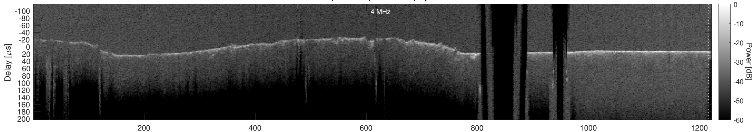
Orbit 16647, Cluttergram
