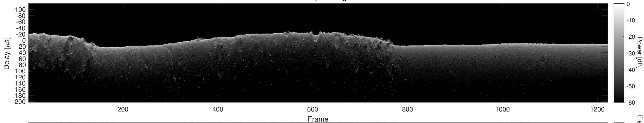
Orbit 16647, Cluttergram
