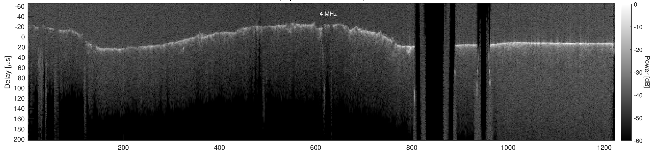
Orbit 16647, Cluttergram
