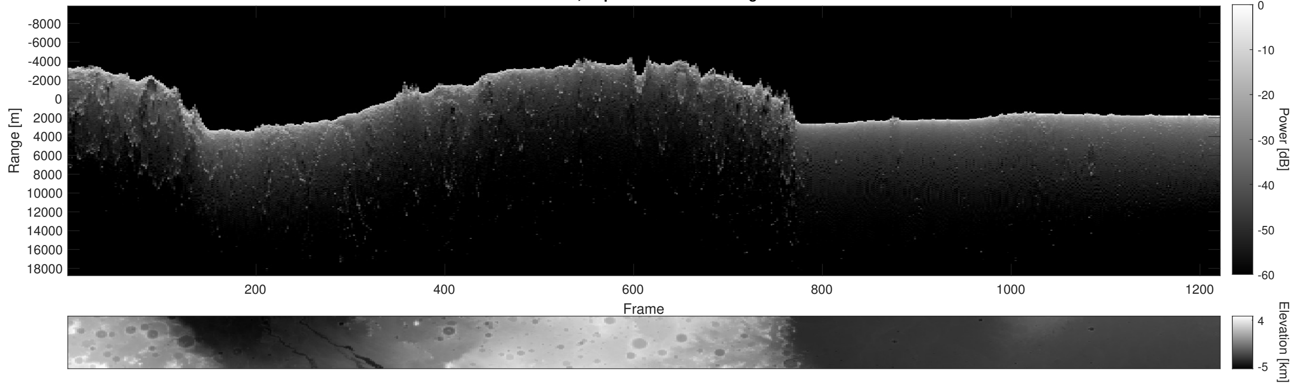
Orbit 16647, Depth-Corrected Cluttergram
