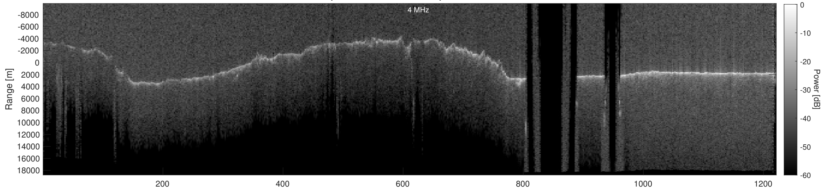
Orbit 16647, Depth-Corrected Cluttergram
