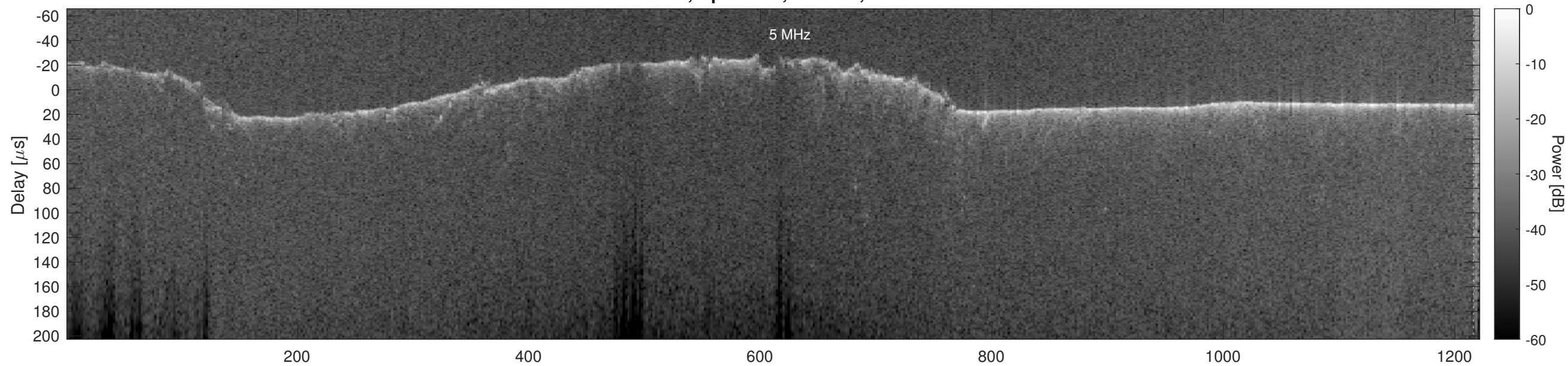
Orbit 16647, Optimized, Window, Channel 2
