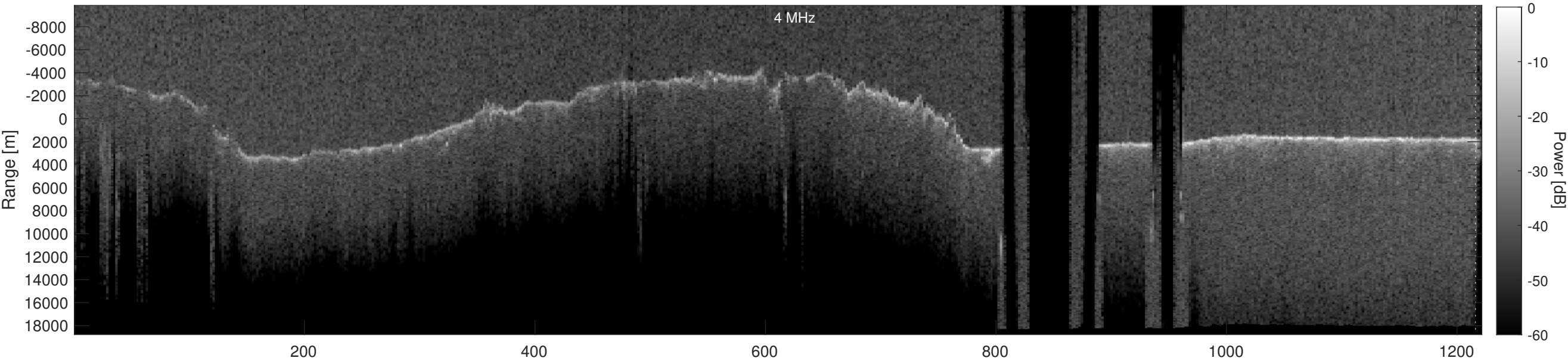
Orbit 16647, Depth-Corrected Cluttergram
