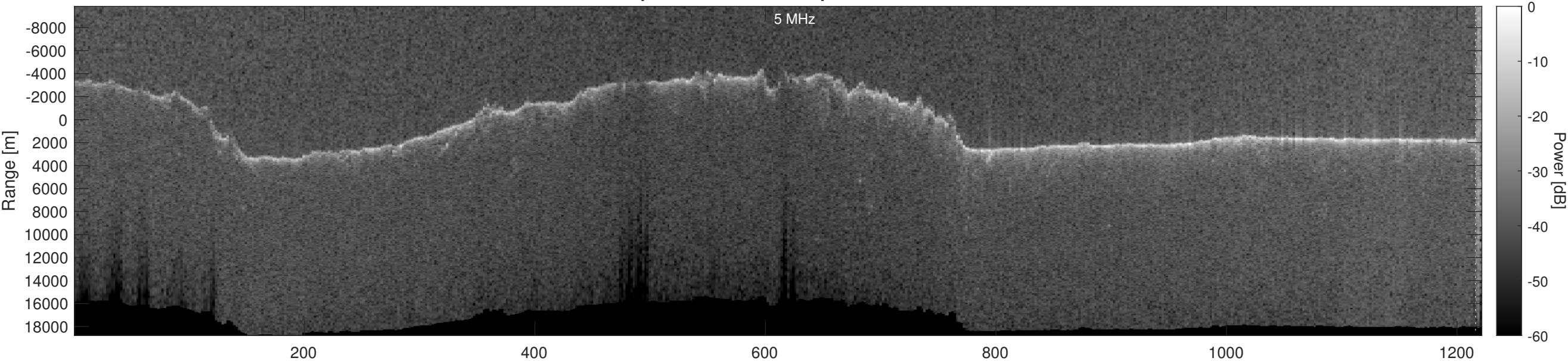
Orbit 16647, Optimized, Window, Depth-Corrected, Channel 2
