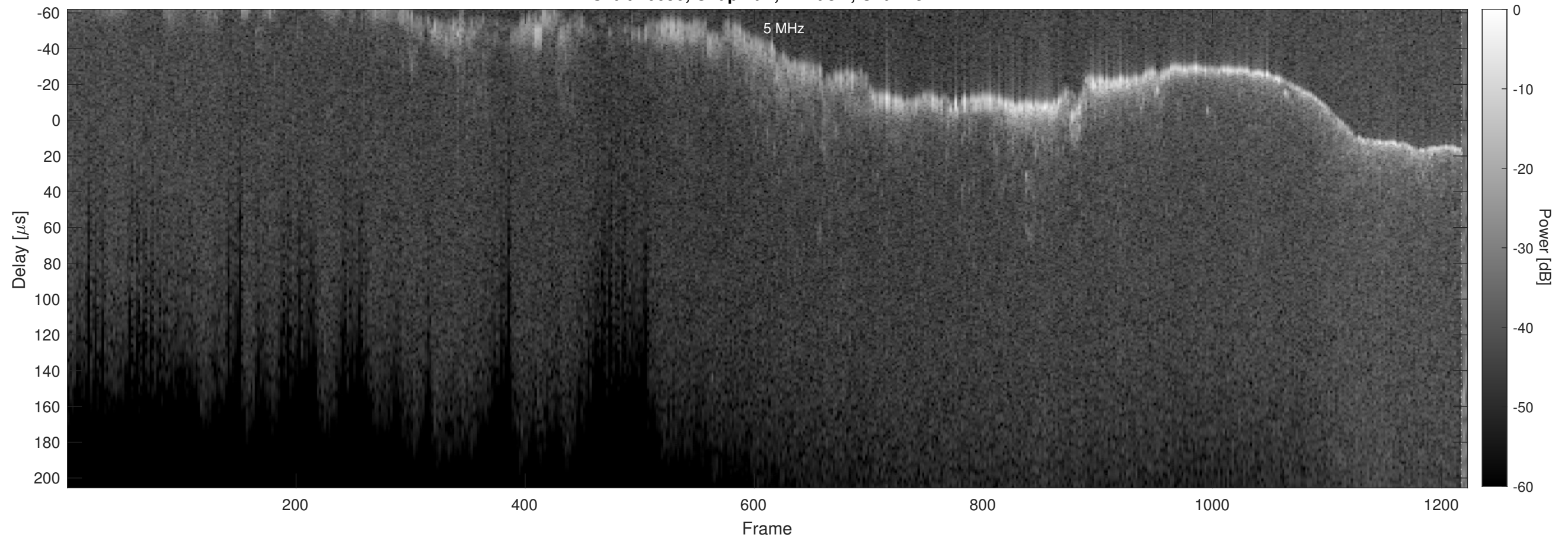
Orbit 16650, Chapman, Window, Channel 2
