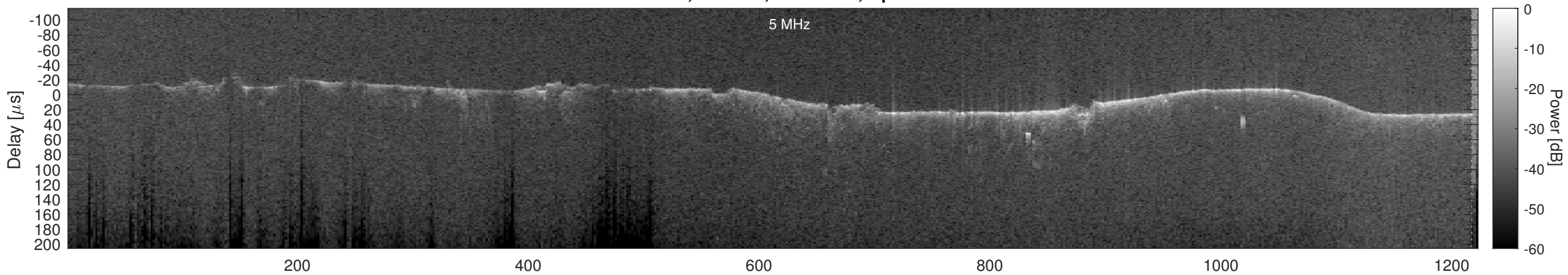
Orbit 16650, Cluttergram
