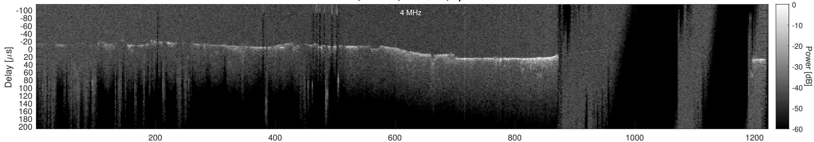
Orbit 16650, Cluttergram
