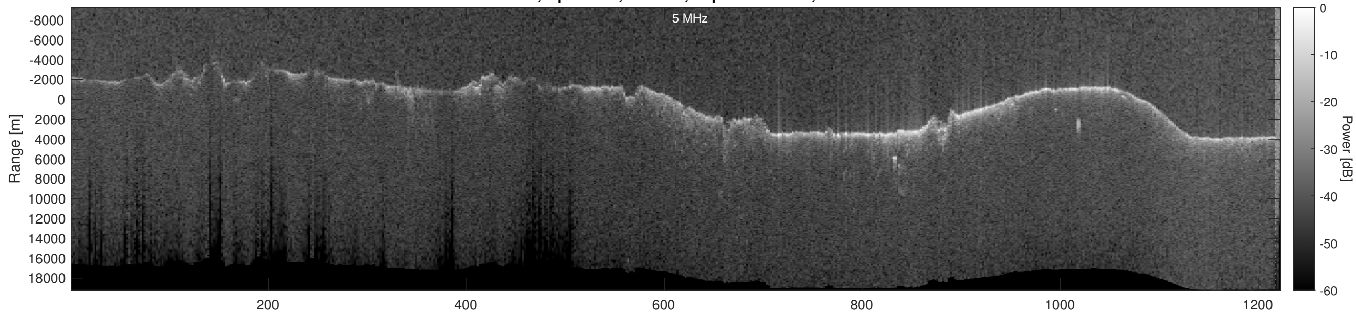
Orbit 16650, Optimized, Window, Depth-Corrected, Channel 2
