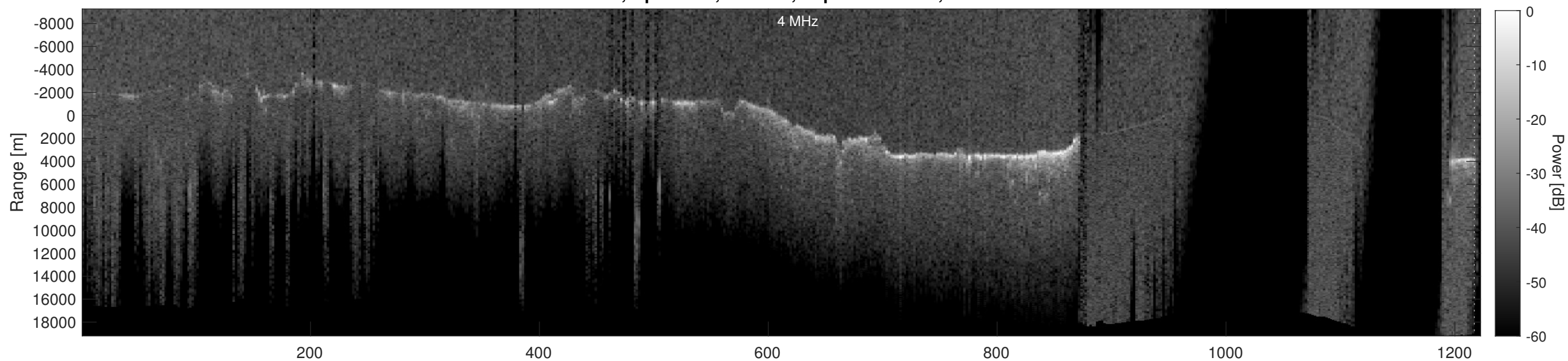
Orbit 16650, Depth-Corrected Cluttergram
