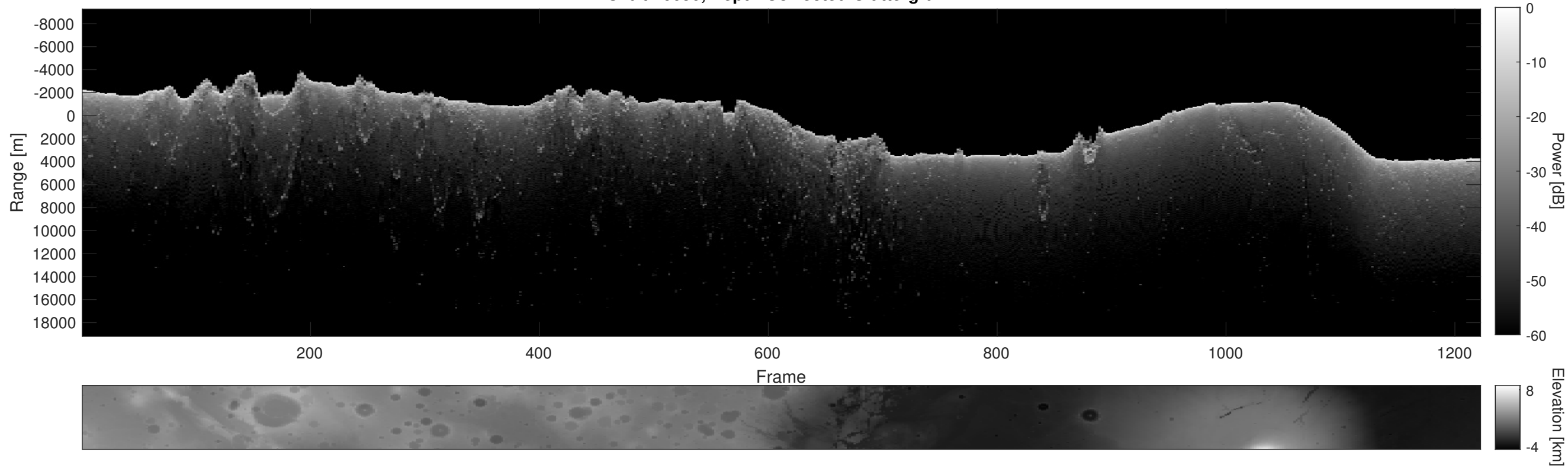
Orbit 16650, Depth-Corrected Cluttergram
