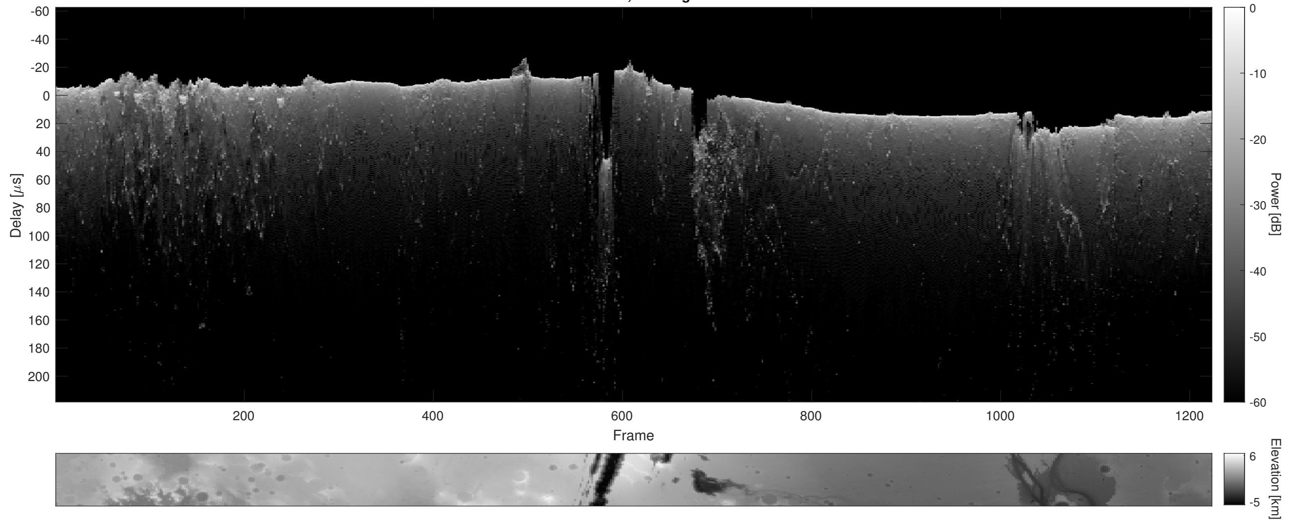
Orbit 16652, Cluttergram
