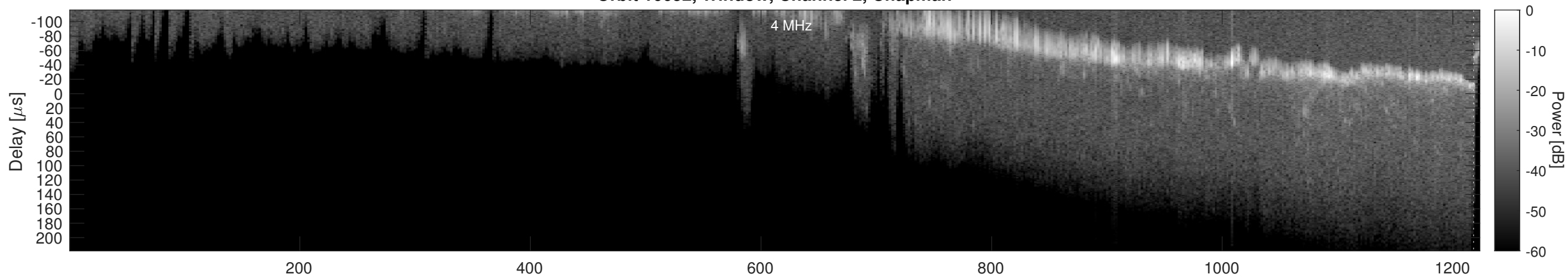
Orbit 16652, Window, Channel 2, Optimized
