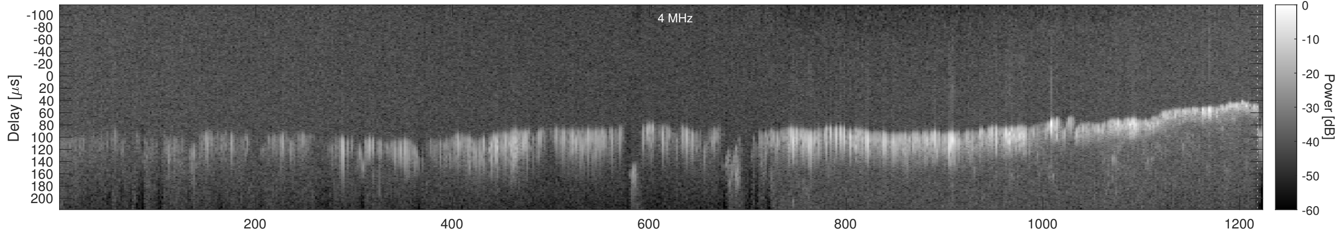
Orbit 16652, Window, Channel 2, Chapman
