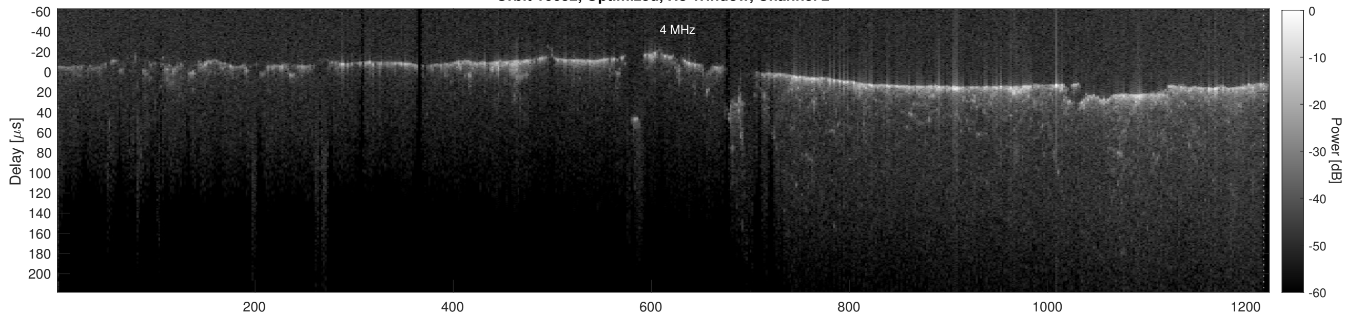
Orbit 16652, Cluttergram
