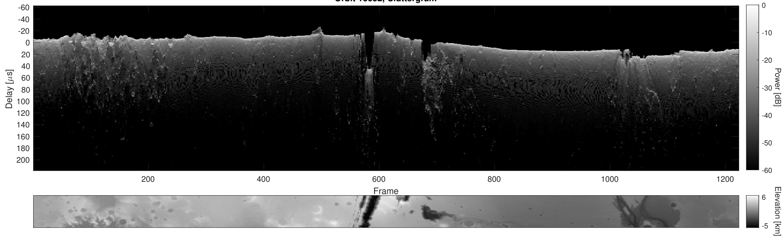
Orbit 16652, Cluttergram
