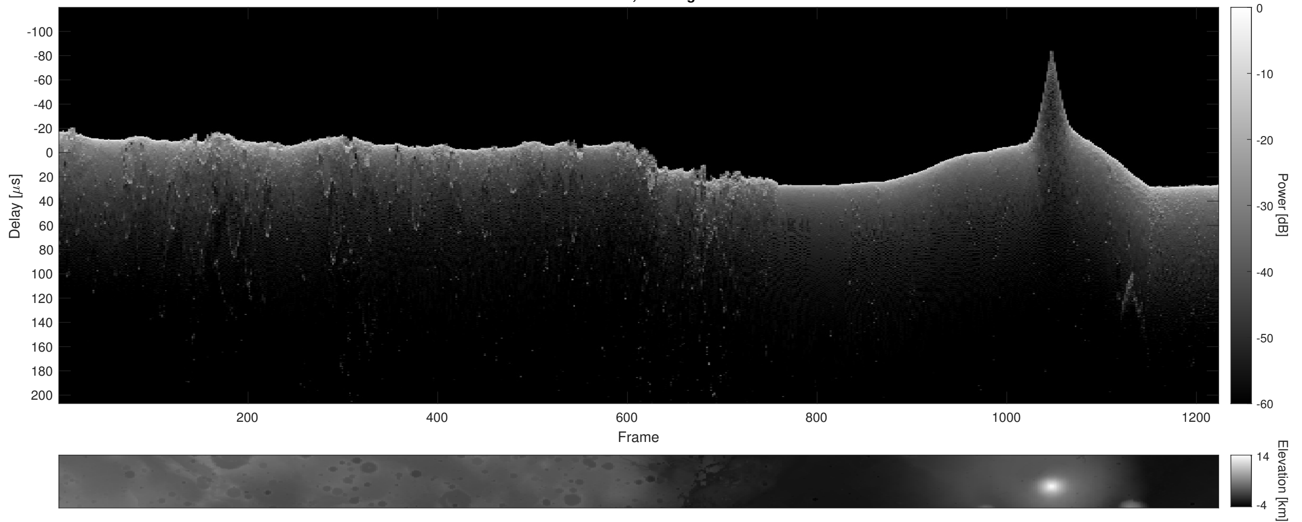
Orbit 16657, Cluttergram
