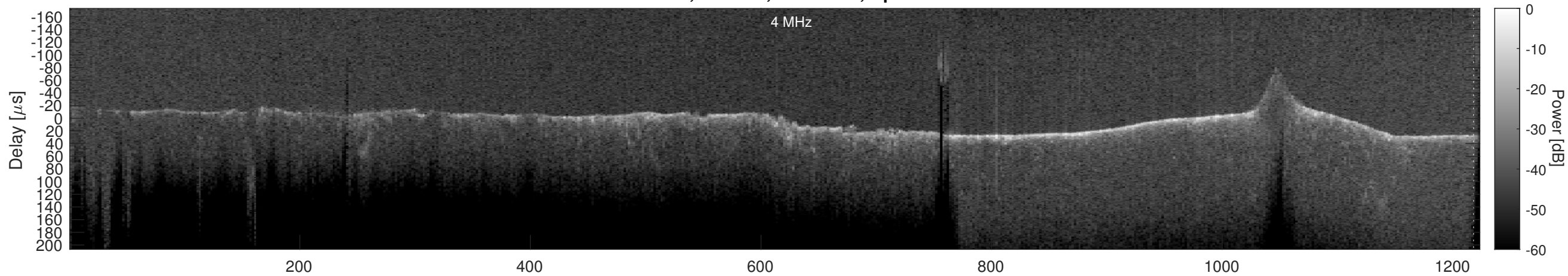
Orbit 16657, Cluttergram
