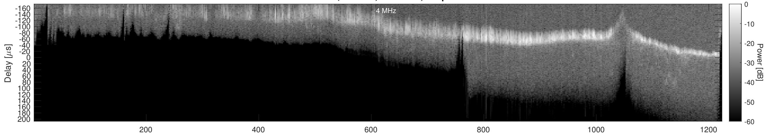
Orbit 16657, Window, Channel 2, Optimized
