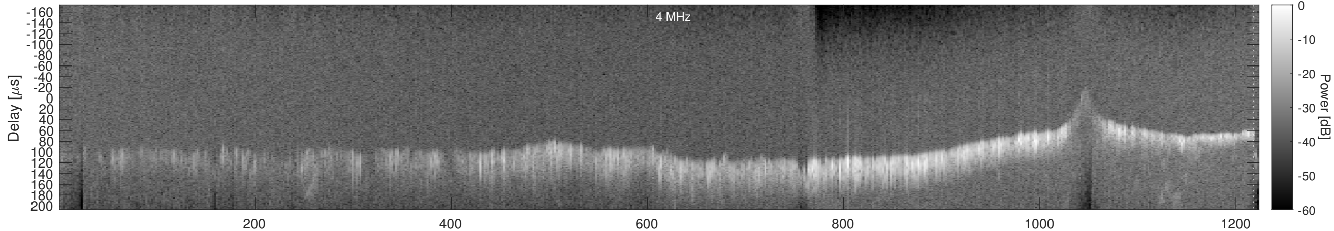
Orbit 16657, Window, Channel 2, Chapman
