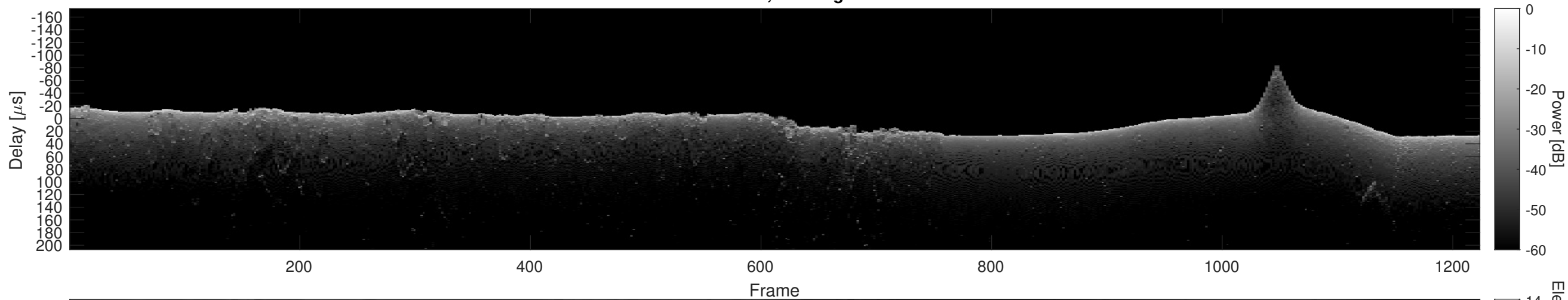
Orbit 16657, Cluttergram
