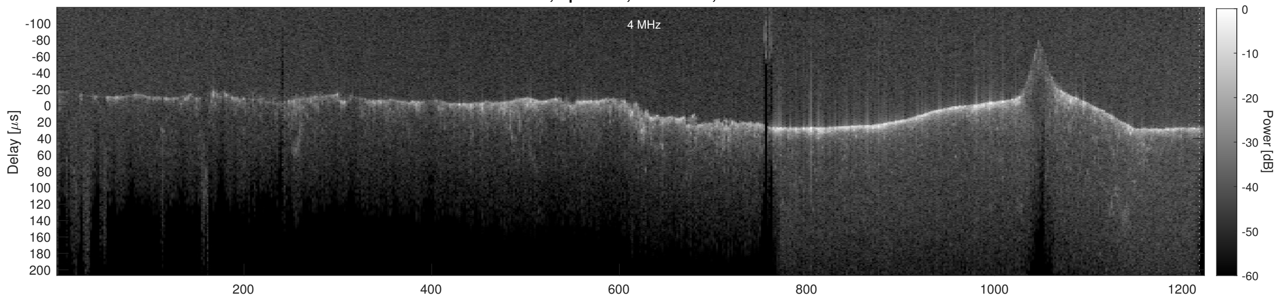
Orbit 16657, Cluttergram
