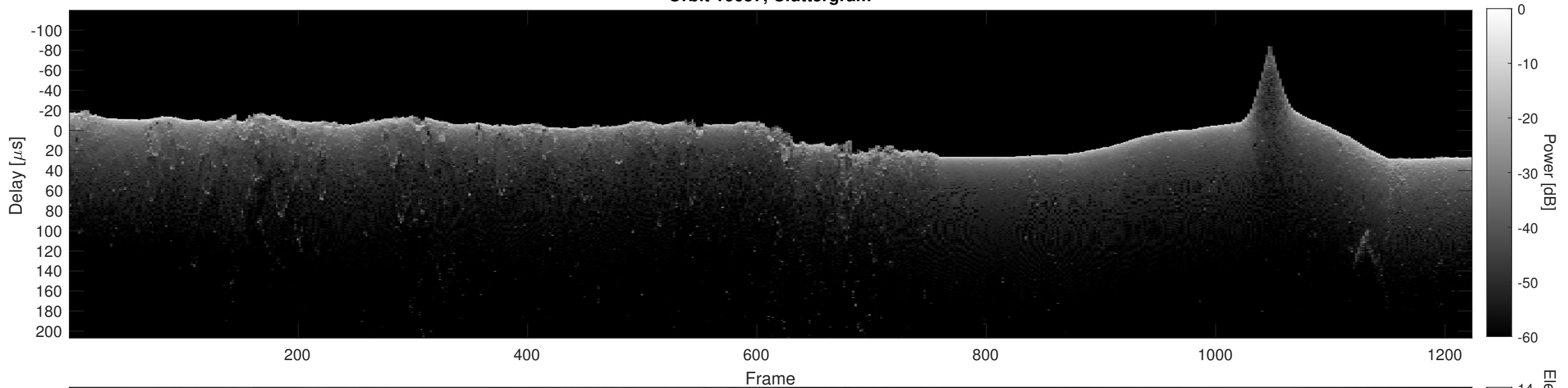
Orbit 16657, Cluttergram
