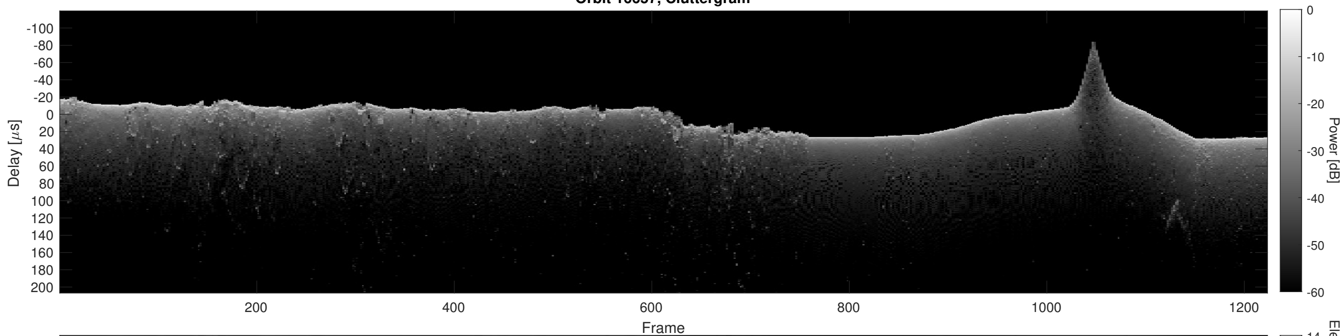
Orbit 16657, Cluttergram
