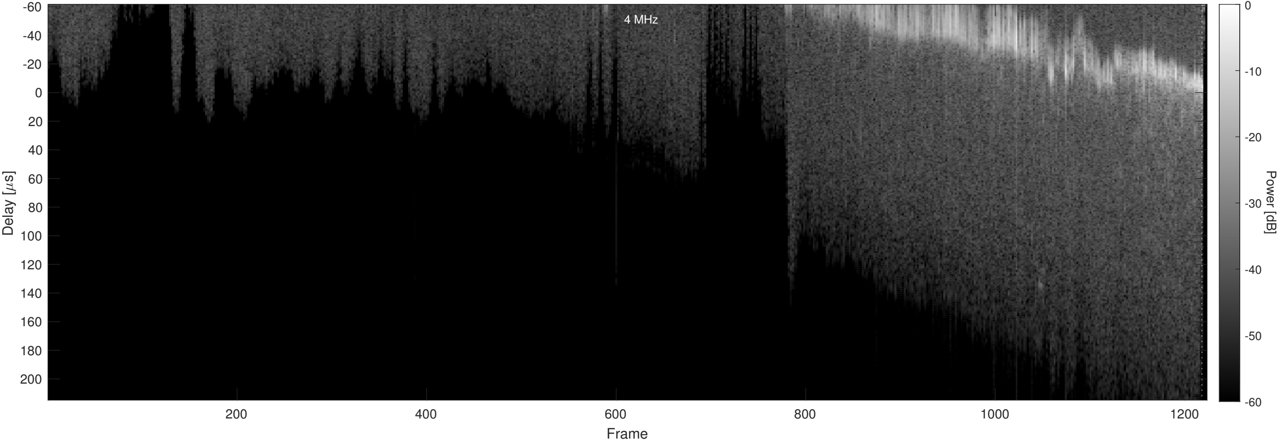
Orbit 16659, Chapman, No Window, Channel 2
