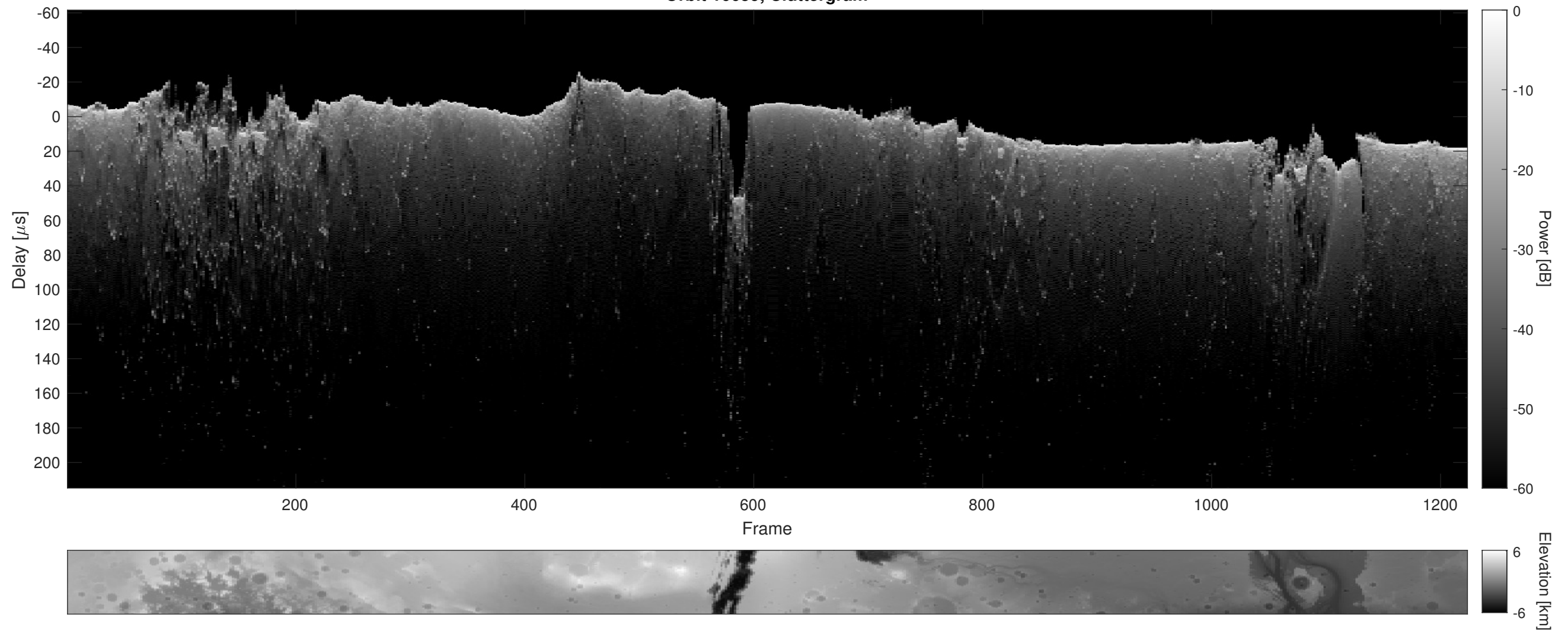
Orbit 16659, Cluttergram
