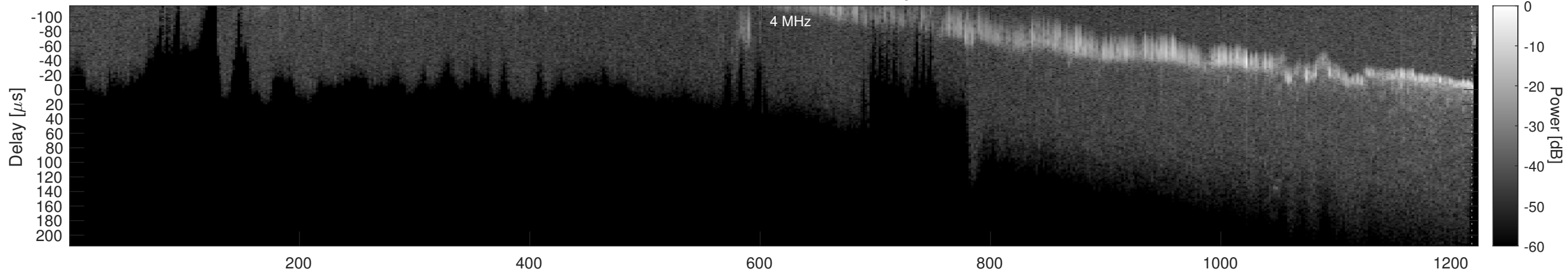
Orbit 16659, Window, Channel 2, Optimized
