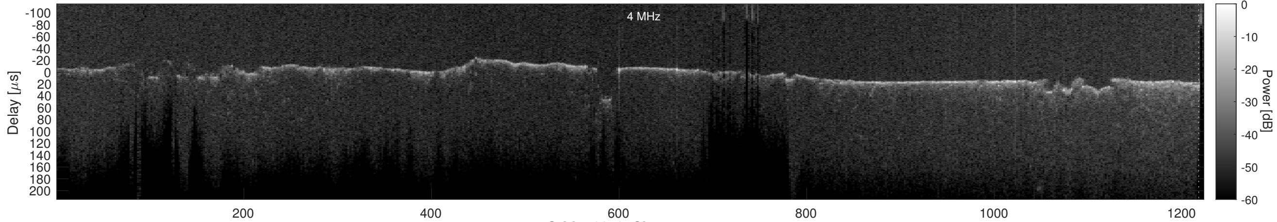
Orbit 16659, Cluttergram
