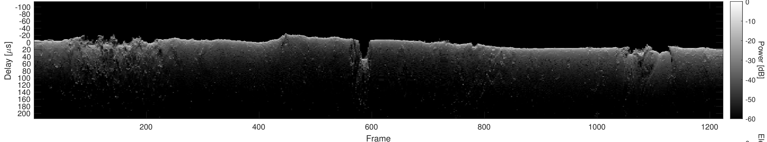
Orbit 16659, Cluttergram
