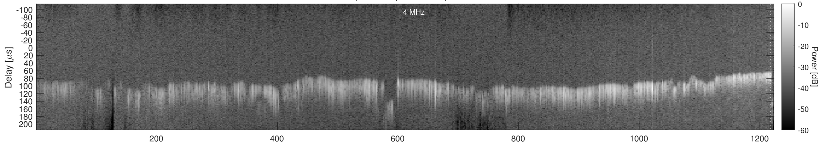
Orbit 16659, Window, Channel 2, Chapman
