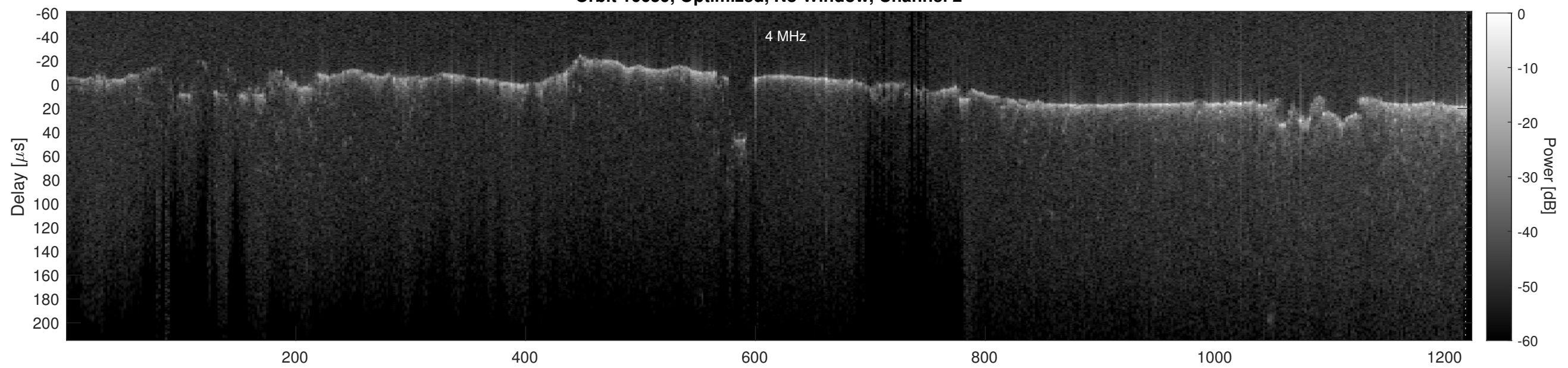
Orbit 16659, Cluttergram
