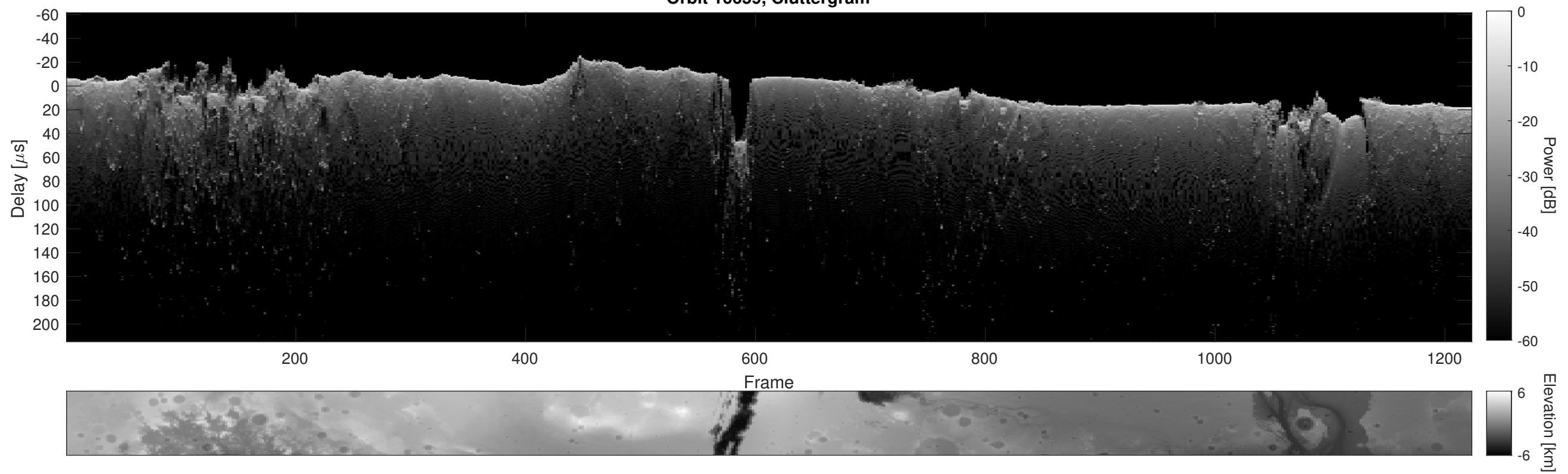
Orbit 16659, Cluttergram
