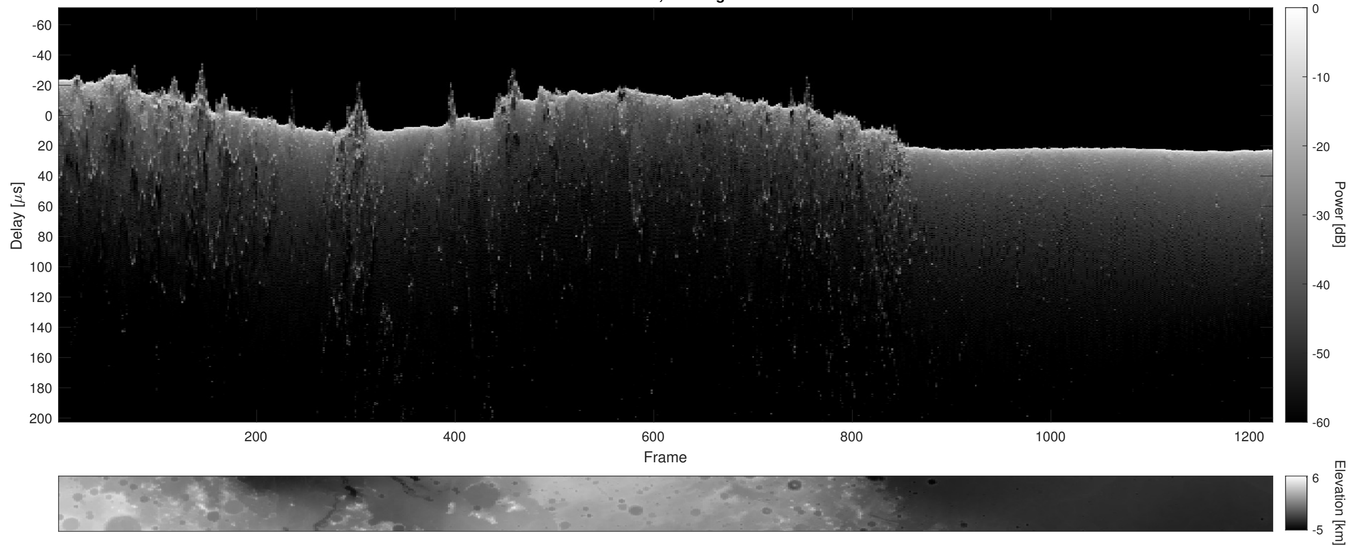
Orbit 16661, Cluttergram
