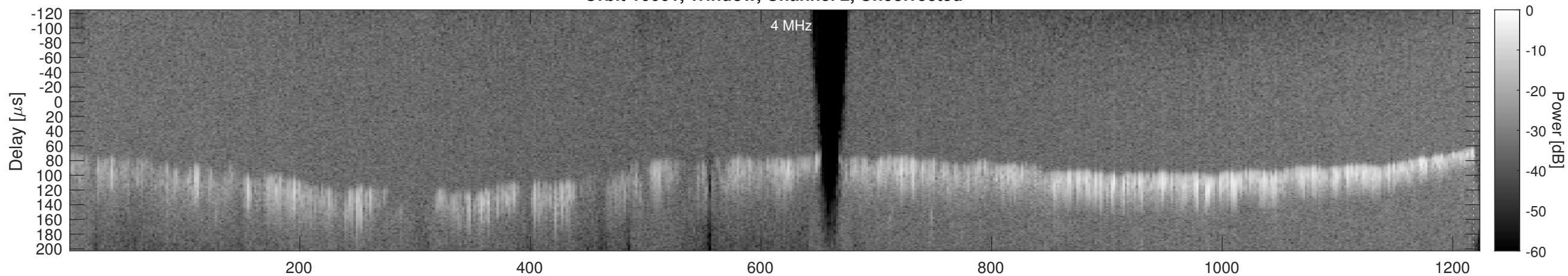
Orbit 16661, Window, Channel 2, Chapman
