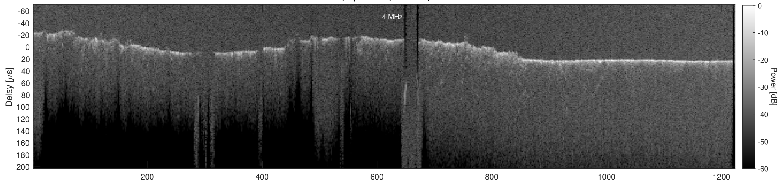
Orbit 16661, Cluttergram
