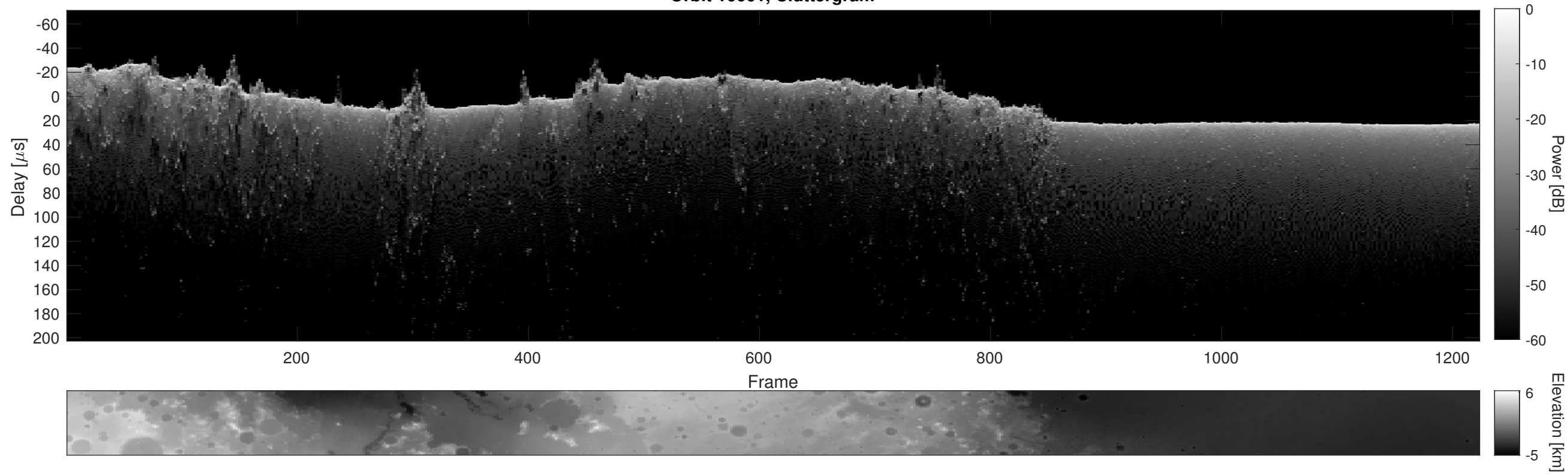
Orbit 16661, Cluttergram
