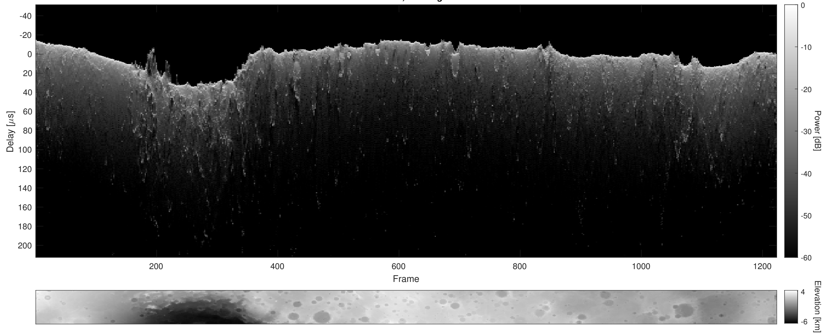
Orbit 16665, Cluttergram
