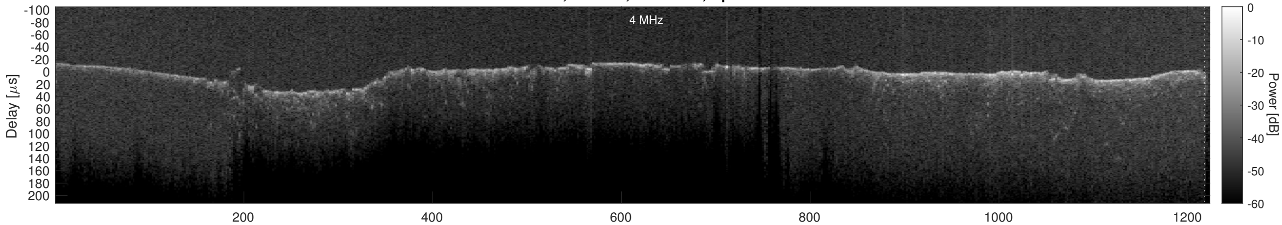
Orbit 16665, Cluttergram
