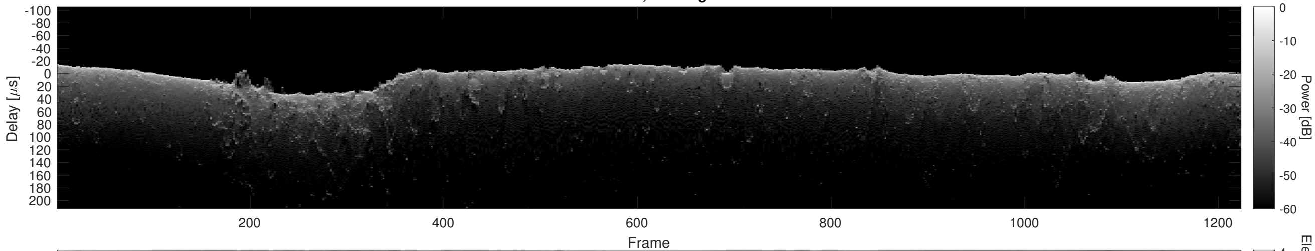
Orbit 16665, Cluttergram
